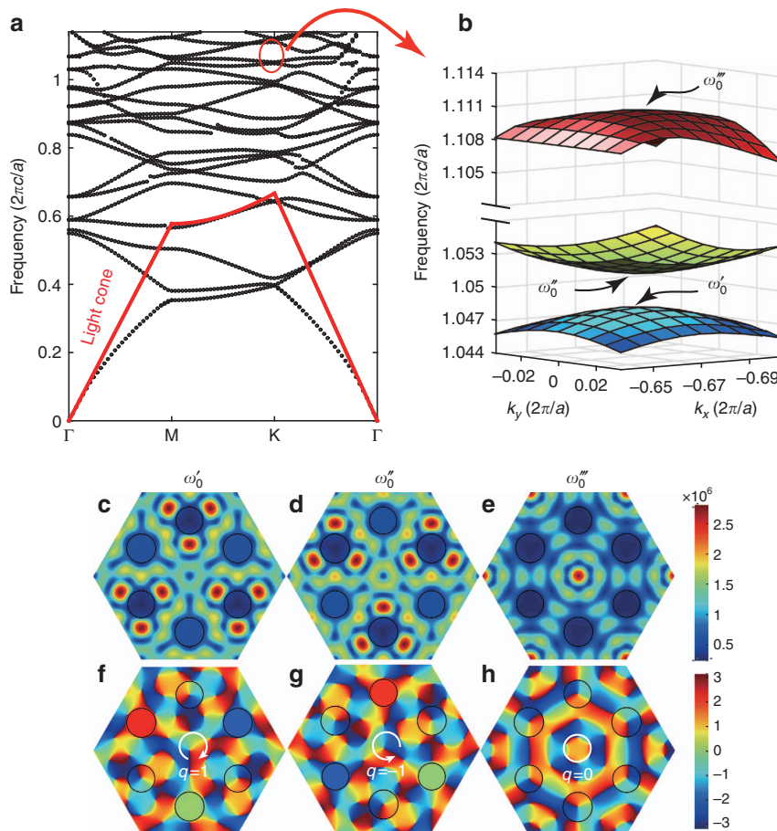
Figure 2 Eigenmodes supported by the 2D photonic lattice. (a) Band structure for the even modes in the SOG. (b) Dispersion relation in the vicinity of the K point (-4\pi/3a, 0) . (c–e) Amplitude ( |H_z| ) distributions on the symmetric plane in the z direction for the eigenmodes at the K point for q=1 ( \omega'_0 = 1.048 \times 2\pi c/a ), q=-1 ( \omega''_0 = 1.052 \times 2\pi c/a ) and q=0 ( \omega'''_0 = 1.110 \times 2\pi c/a ), respectively. (f–h) Phase distributions ( \arg(H_z) ) of the three modes that correspond to q=+1, -1 and 0 , respectively.
