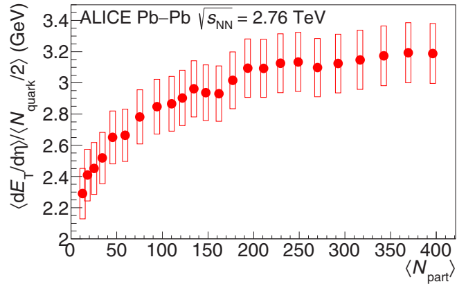
FIG. 9. Measurements of \langle dE_T/d\eta \rangle / \langle N_{quark}/2 \rangle versus \langle N_{part} \rangle at midrapidity in Pb-Pb collisions at \sqrt{s_{NN}} = 2.76 TeV. Note the suppressed zero. The boxes indicate the systematic uncertainties.
