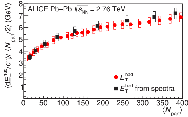
FIG. 3. Comparison of \langle dE_T^{\text{had}}/d\eta \rangle / \langle N_{\text{part}}/2 \rangle versus \langle N_{\text{part}} \rangle from the measured particle spectra and as calculated from the tracking detectors. The boxes indicate the systematic uncertainties.
