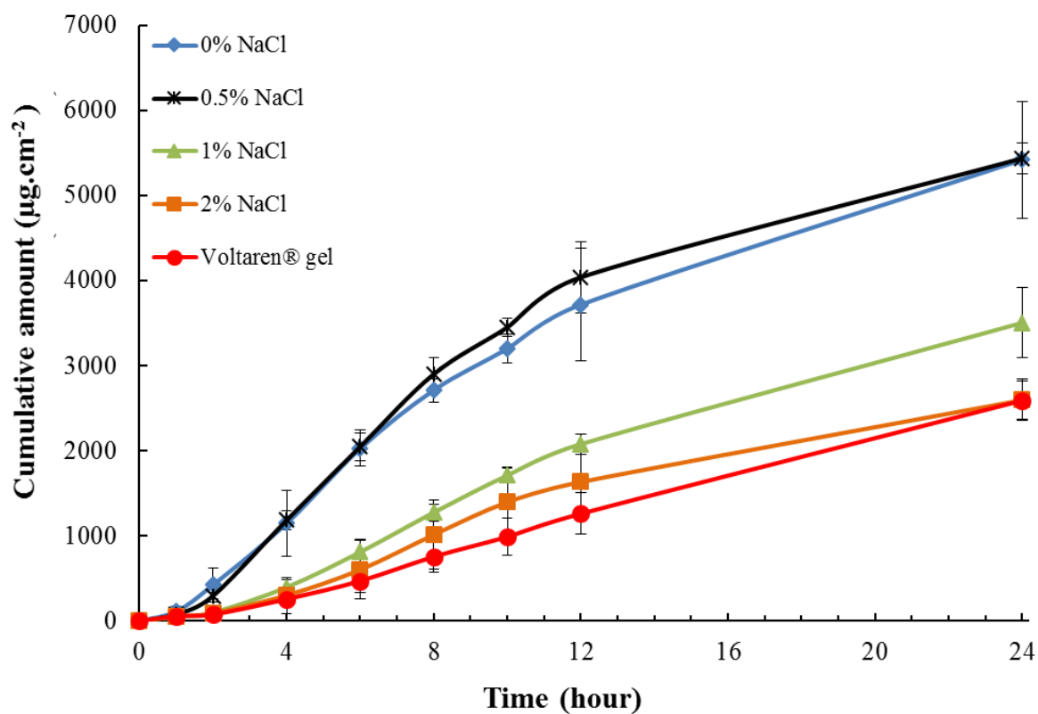
Figure 7 Cumulative amount \mu\text{g}\cdot\text{cm}^{-2} of diclofenac sodium permeated from 1 % w/w 50:50 LA HA gellan fluid gels prepared at different NaCl concentrations compared with Voltaren® gel. Values are represented as mean \pm SD (n=3).
