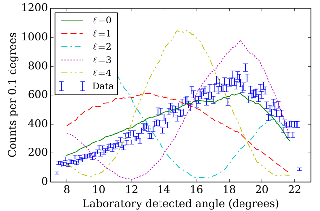
FIG. 7. (Color online) Angular distribution for the state at 18.14 MeV (points with error bars), with simulated distributions (lines).
