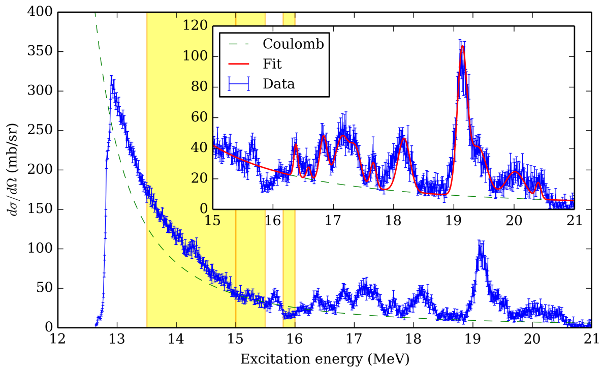
FIG. 3. (Color online) Excitation energy in ^{28}\text{Mg} , showing the calculated Rutherford cross section (green dashed line) that has been used for normalization. The inset shows detail of the resonances with a fit using overlaid Gaussian peak shapes (red solid line). The three regions that were used for normalization of the data are indicated with yellow shading. See text for details.
