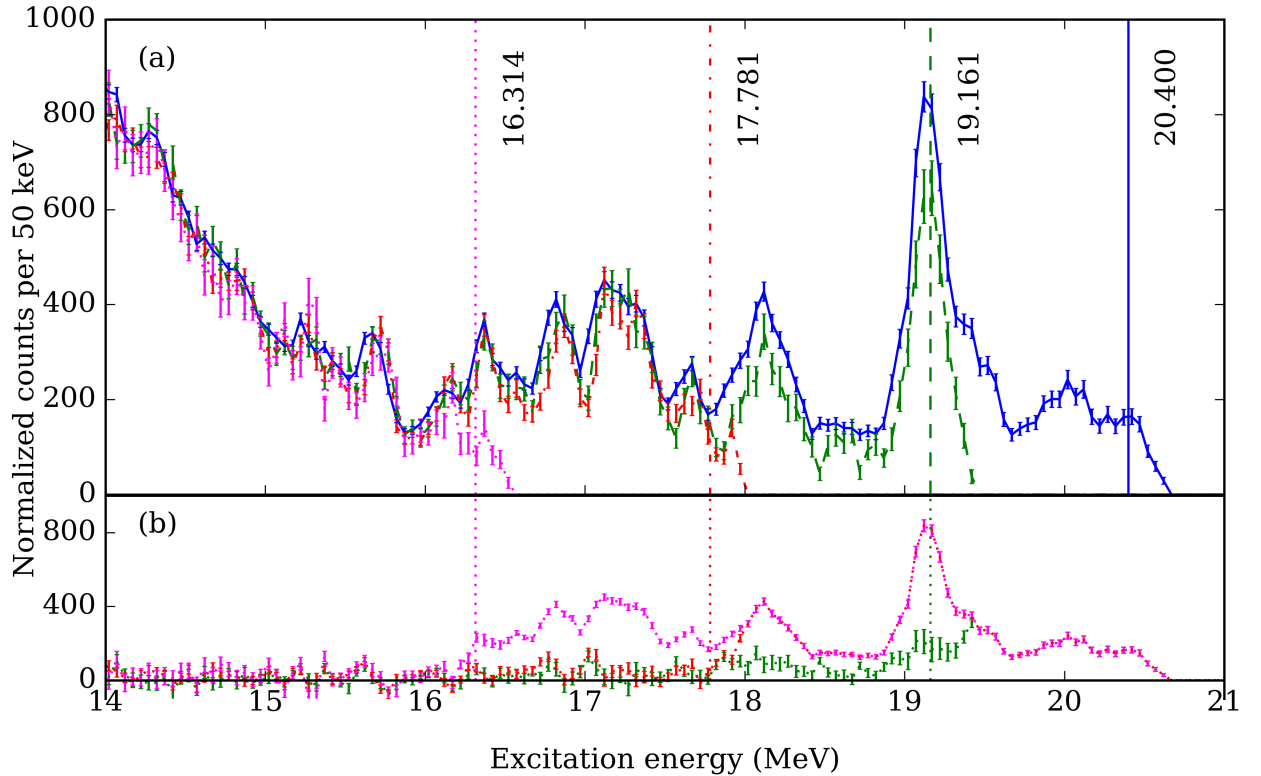
FIG. 4. (Color online) Comparison of excitation functions for ^{28}\text{Mg} measured with four different beam energies, showing (a) the spectra normalised to each other using the Rutherford cross section between 13.1 and 14.0 MeV and (b) the differences between each of the lower beam energy spectra (green with dashed line, red with dot-dashed line, magenta with dotted line) and the spectrum with the highest beam energy (blue with solid line). For each spectrum, the highest available excitation energy is marked.
