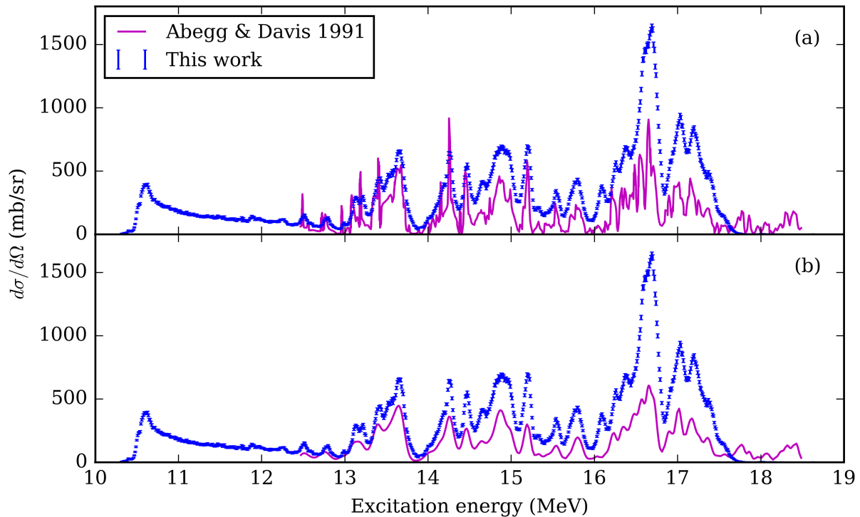
FIG. 2. (Color online) Comparison of the excitation function of ^{24}\text{Mg} measured in this work at 180^\circ and of Ref. [25] measured at 168^\circ . The latter is shown (a) unaltered, and (b) after convolution with a resolution of 60 keV FWHM.
