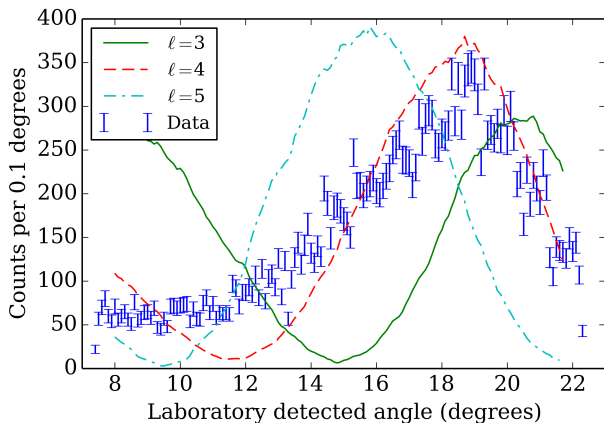
FIG. 6. (Color online) Angular distribution for the state at 19.14 MeV (points with error bars), with simulated distributions (lines).
