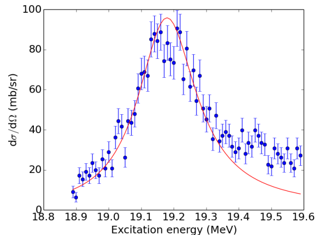
FIG. 8. (Color online) R -Matrix fit (red line) to the state (blue circles) at 19.14 MeV with J^\pi = 4^+ . A clear shoulder on the high energy side of the peak has been ignored in the fit. In the fitting region ( E_x = 18.9 – 19.3 MeV) \chi^2/\text{d.o.f} = 1.22
