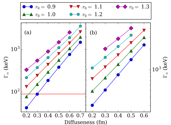
FIG. 9. (Color online) Calculated widths for the \alpha and neutron channels, (a) \Gamma_\alpha and (b) \Gamma_n , using the code Gamow , as a function of the radius and diffuseness parameters r_0 and a . A horizontal red line shows the experimental value of \Gamma_\alpha (90 keV); the corresponding value for \Gamma_n found using an R -Matrix calculation (150 keV) is not visible on this scale.
