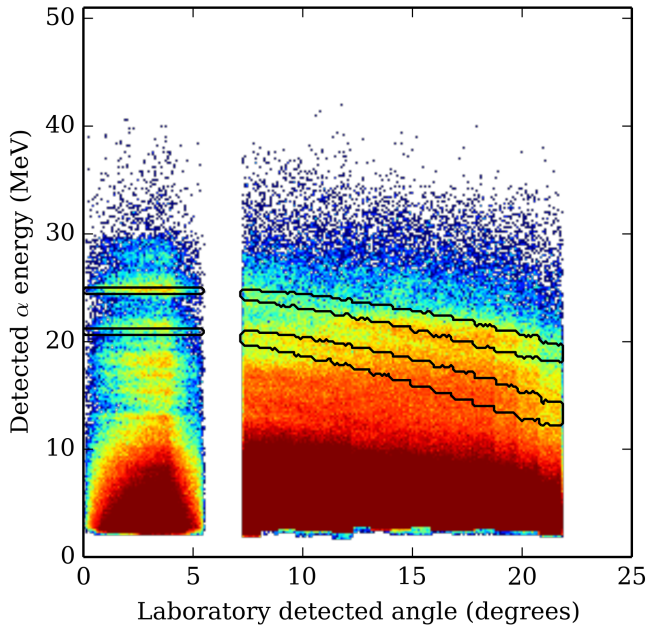
FIG. 5. (Color online) Energy of all \alpha -particles from ^{28}\text{Mg} plotted against angle, measured with the coordinate origin placed at the entrance window. The data in the left-hand block are from the zero-degree detector, and those in the right-hand block are from the lampshade array. The software gates used to obtain angular distributions are shown; see text for details of the gating procedure.
