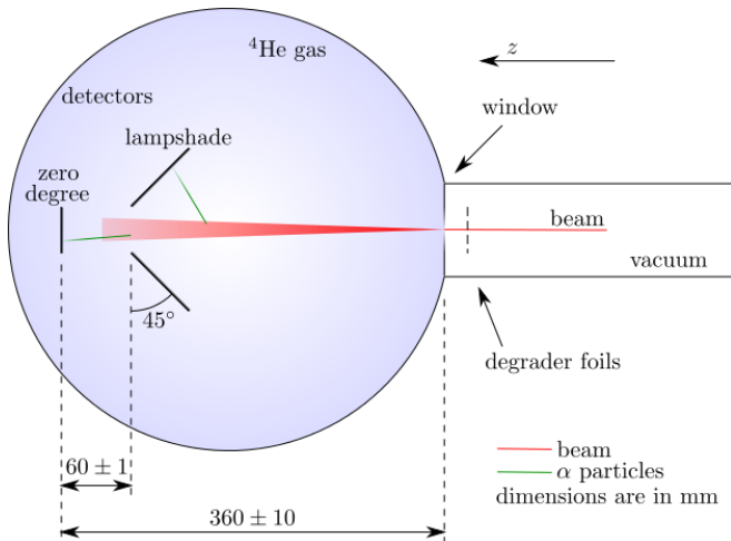
FIG. 1. (Color online) Schematic of the experimental chamber.
