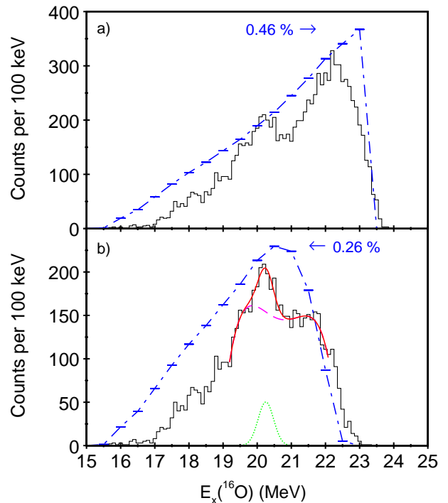
FIG. 7: (Color online) Excitation energy for the ^{12}\text{C}^*[7.65 \text{ MeV}] + \alpha decay of c from a) all events in the present data and b) events with E_x(^9\text{Be}) \geq 3.5 MeV. The (blue) dot-dash lines represent the detection efficiency profiles, for which the peak values are given. In b) the results of a Gaussian peak fit are shown (see text).
