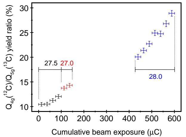
FIG. 9: (Color online) Total energy spectrum (Fig. 1) Q_{4g}(^{12}\text{C}) to Q_{5g}(^{13}\text{C}) yield ratio as a function of cumulative beam exposure. The beam energies of 27.0 (red points), 27.5 (black points) and 28.0 MeV (blue points), at which the data points were obtained, are noted.
