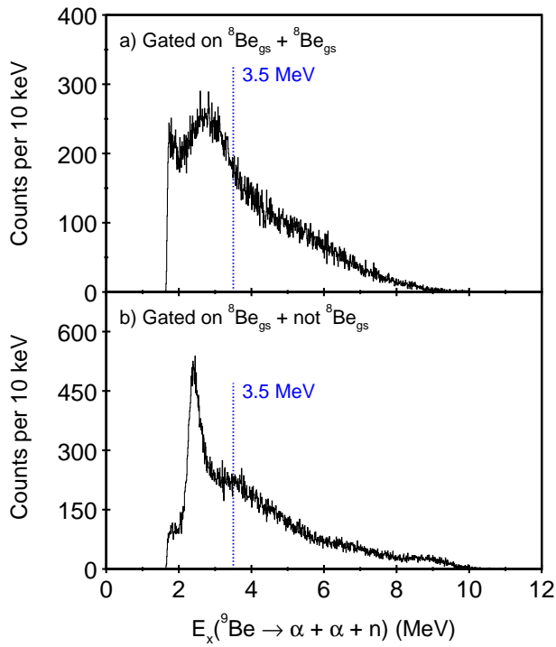
FIG. 4: (Color online) Excitation energy for {}^9\text{Be} \rightarrow \alpha + \alpha + n at a beam energy of 28.0 MeV. In (a) the data are gated on two {}^8\text{Be} ground state pairs and in (b) on one {}^8\text{Be} ground state pair and one pair not in the {}^8\text{Be} ground state. The (blue) dotted vertical line indicates the energy of the 3.5 MeV gate applied to the data (see text).
