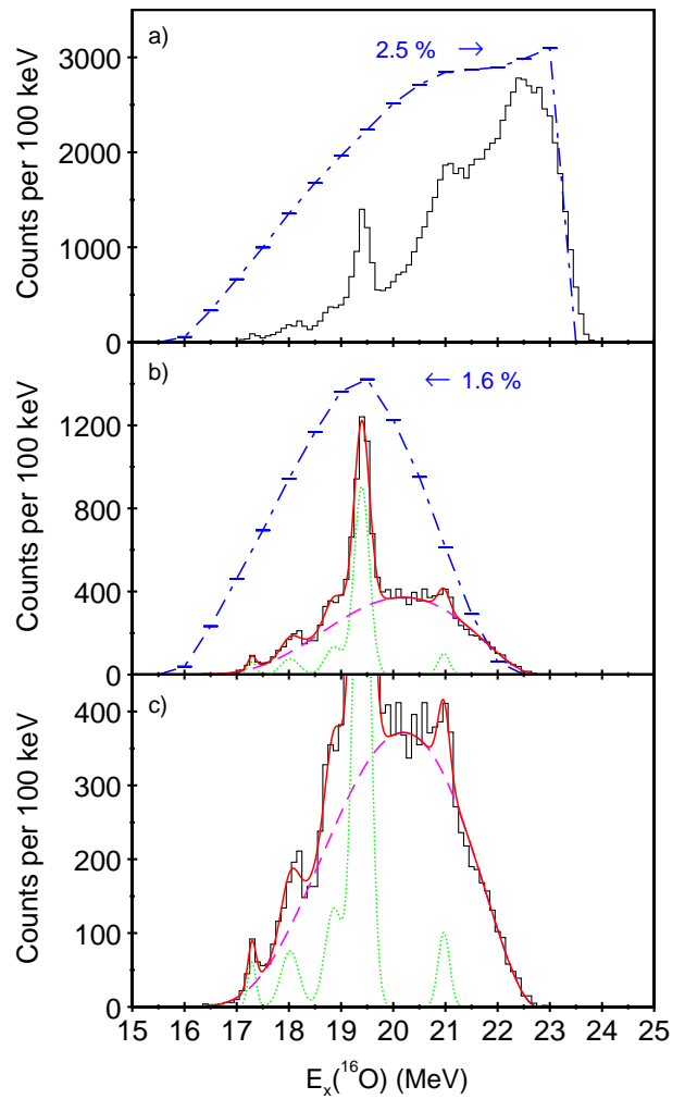
FIG. 5: (Color online) Excitation energy for the {}^8\text{Be}_{\text{gs}} + {}^8\text{Be}_{\text{gs}} decay of {}^{16}\text{O} from a) all events in the present data and b) and c) events with E_x({}^9\text{Be}) \geq 3.5 MeV. The (blue) dot-dash lines represent the detection efficiency profiles, for which the peak values are given. In b) and c) the results of a Gaussian peak fit are shown (see text).
