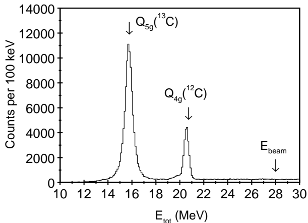
FIG. 1: Total energy spectrum at a beam energy of 28.0 MeV. The expected positions of peaks corresponding to the ^{13}\text{C}(^4\text{He}, \alpha\alpha\alpha\alpha)n and ^{12}\text{C}(^4\text{He}, \alpha\alpha\alpha)\alpha reactions are labelled as Q_{5g}(^{13}\text{C}) and Q_{4g}(^{12}\text{C}) , respectively.
