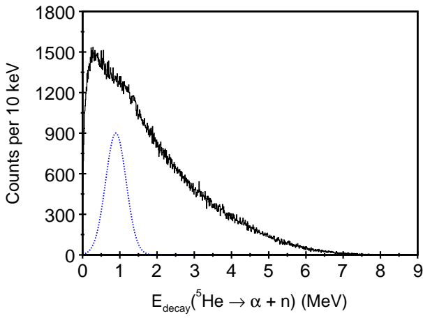
FIG. 2: (Color online) Decay energy for {}^5\text{He} \rightarrow \alpha + n at a beam energy of 28.0 MeV. The (blue) dotted Gaussian line shape indicates the expected position (0.894 MeV) and FWHM (0.648 MeV) of the {}^5\text{He} ground state.
