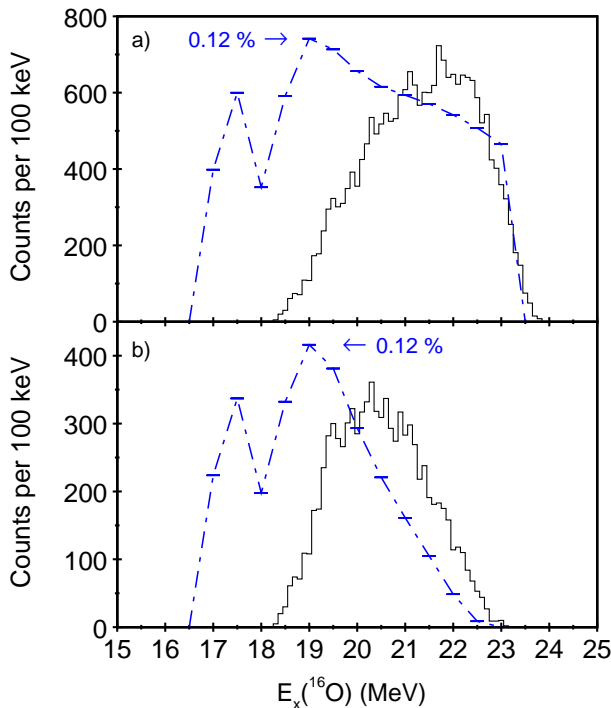
FIG. 8: (Color online) Excitation energy for the ^{12}\text{C}^*[9.64 \text{ MeV}] + \alpha decay of ^{16}\text{O} from a) all events in the present data and b) events with E_x(^9\text{Be}) \geq 3.5 \text{ MeV} . The (blue) dot-dash lines represent the detection efficiency profiles, for which the peak values are given.
