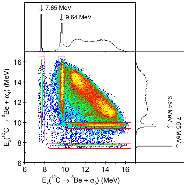
FIG. 6: (Color online) Excitation energy in ^{12}\text{C} obtained from E_{\text{decay}}(^8\text{Be}_{\text{gs}} + \alpha_3) against that obtained from E_{\text{decay}}(^8\text{Be}_{\text{gs}} + \alpha_4) , for ^8\text{Be}_{\text{gs}} + \text{not } ^8\text{Be}_{\text{gs}} events. The (red) boxes in the main panel indicate the windows used to select the 7.65 and 9.64 MeV states. In the upper and right panels the X and Y projections of the data are shown. The beam energy was 28.0 MeV.
