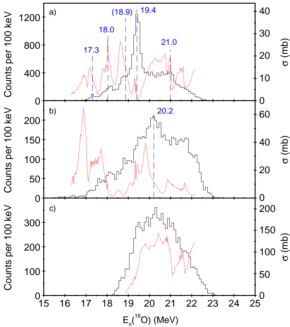
FIG. 11: (Color online) Excitation energy obtained from the ^{13}\text{C}(^4\text{He},4\alpha)\text{n} breakup reaction (solid (black) lines and left hand Y-scale) and ^{12}\text{C}(^4\text{He},4\alpha) excitation functions of Curtis et al. [21] (dotted (red) lines and right hand Y-scale), for the a) ^8\text{Be}_{\text{gs}} + ^8\text{Be}_{\text{gs}} , b) ^{12}\text{C}^*[7.65 \text{ MeV}] + \alpha and c) ^{12}\text{C}^*[9.64 \text{ MeV}] + \alpha decay of ^{16}\text{O} . The vertical (blue) dashed lines indicate the energies (in MeV) of the fitted peaks and features (see text).
