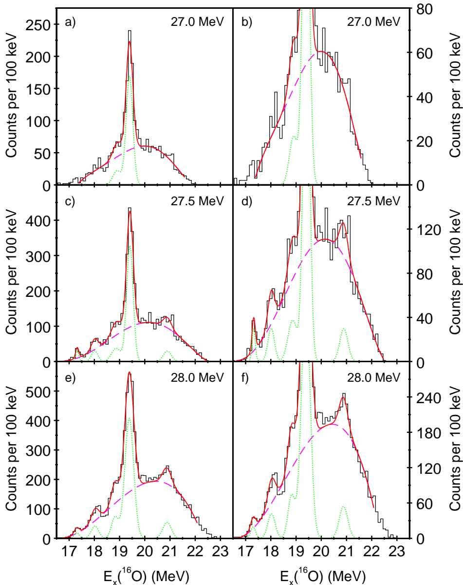
FIG. 10: (Color online) Excitation energy for the {}^8\text{Be}_{\text{gs}} + {}^8\text{Be}_{\text{gs}} decay of {}^{16}\text{O} , at beam energies of a) and b) 27.0, c) and d) 27.5, and e) and f) 28.0 MeV. In a), c) and e) the full spectra are shown, whereas in b), d) and f) the Y-scale has been expanded. In all panels the results of a Gaussian peak fit are shown (see text).
