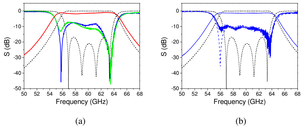
Figure 3. Measured and simulated filter responses. (a) The initially assembled device. (2) The device after a compression resulting in its height reduced from 1.095 mm to 1.085 mm.
