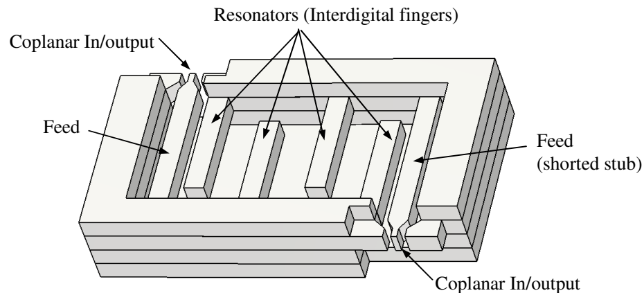
Figure 1. Diagram of the interdigital filter, with the top layer removed to assist viewing.
