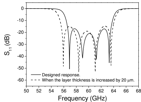
Figure 4. Modelling of the contribution of possible fabrication errors to the filter responses.
