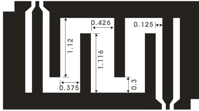
Figure 2. Some dimensions of the middle layer of the filter. Dimensions in millimetres.
