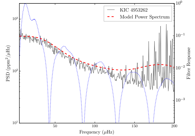
Figure 5. Filter response overlotted on KIC 4953262 power spectrum. Clearly most of the signal involved in the construction of the noise metric appears in the region 0 < \nu \lesssim 40 \mu\text{Hz} . The filter response is shown on a log scale to emphasise regions of the power spectrum that contribute to the noise metric.
