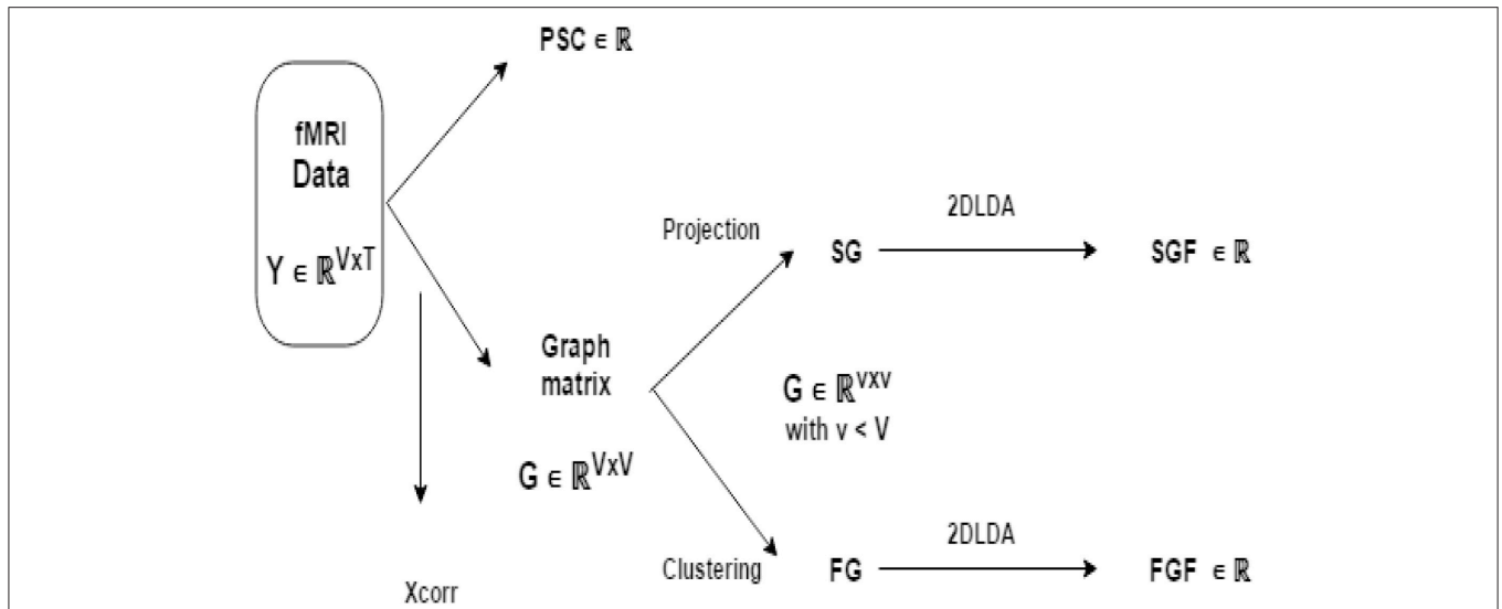
FIGURE 1 | Illustration of fMRI feature generation pipeline: from BOLD signal data Y to three fMRI features (PSC, FGF, and SGF). FG and SG are the reduced version of graph matrix G via functional grouping and spatial grouping (respectively). Note that FGF and SGF are both discriminative features extracted from FG and SG in a supervised manner using 2D-LDA (that is, Linear Discriminant Analysis operating on matrices).
