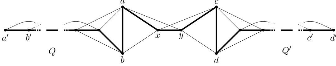
Figure 3: A tail-flexible path Q and head-flexible path Q' with [Q]_2^+ = ab and [Q']_2^- = cd and adjacent vertices x \in N^3(a, b, c) \subseteq T_{ab} and y \in N^3(a, c, d) \subseteq T_{cd} . The thick line represents the ordering of a square path with vertex set V(Q) \cup V(Q') \cup \{x, y\} .
