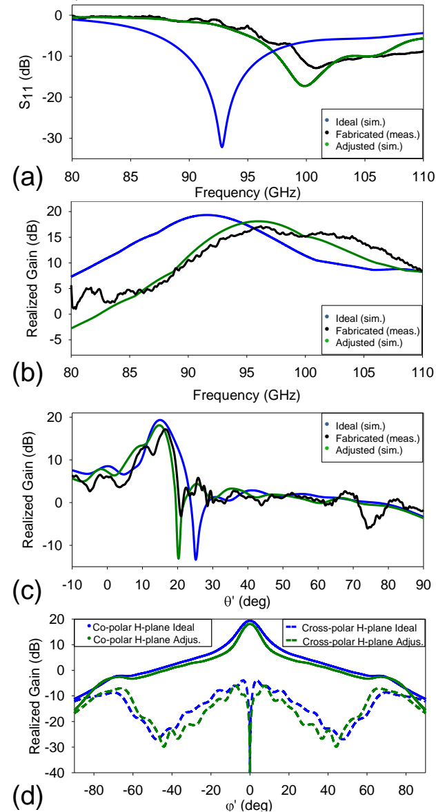
Fig. 3. Return loss (a), realized gain (b) and E-plane radiation diagram at the frequency of the maximum gain (c) for the simulated ideal (blue curves), experimentally measured (black curves) and simulated adjusted (green curves) antenna. Co-polar (continuous line) and cross-polar (dashed line) H-plane radiation diagrams at the frequency of the maximum gain for simulated ideal (blue curves) and adjusted (green curves) antennas (d).
