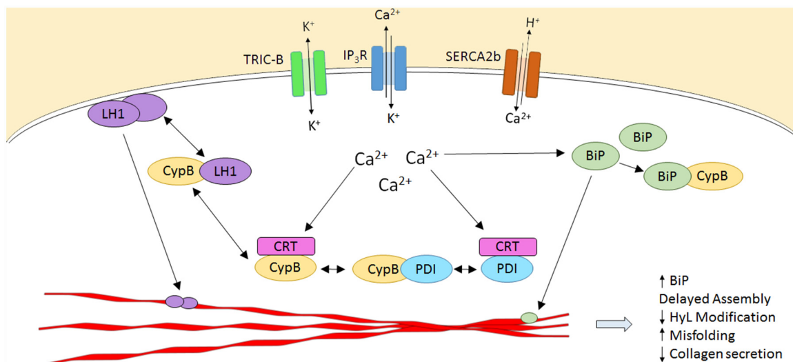
Fig 8. Calcium flux regulates collagen post-translational interactions within the ER. Secreted proteins such as collagen are synthesized within the ER, which contains the major intracellular Ca^{2+} store. In response to extracellular stimuli, Ca^{2+} is released from the ER lumen into the cytoplasm via IP_3 and ryanodine receptors. Cytoplasmic Ca^{2+} that does not bind signaling proteins involved in gene expression is transported back into the ER via SERCA pumps. The continuous fluctuations in free [Ca^{2+}] to and from the ER are indirectly regulated by TRIC channel activity, which mediates transmembrane K^+ flux to maintain electroneutrality across the ER membrane. In fibroblasts and osteoblasts, ER-resident Ca^{2+} -binding chaperones, including BiP, CypB, PDI and calreticulin (CRT), directly interact with collagen alpha chains (red polypeptides) to facilitate or catalyze specific modifications required for assembly and folding. In the absence of TRIC-mediated K^+ flux, Ca^{2+} -dependent “cycling” of these chaperones between inactive, sequestered forms and active, substrate-interacting forms, is dysregulated. Thus, absence of TRIC-B alters ER luminal [Ca^{2+}] , affecting synthesis and secretion of collagen, as well as interactions of collagen-specific chaperones with each other and with their substrate, resulting in abnormal collagen assembly and post-translational modification. BiP, GRP78; CypB, cyclophilin B; CRT, calreticulin; IP_3R , inositol triphosphate receptor; LH1, lysyl hydroxylase 1; PDI, protein disulfide isomerase; SERCA2b, sarcoplasmic-endoplasmic reticulum Ca^{2+} -ATPase isoform 2b; TRIC-B, trimeric intracellular cation channel subtype B.
