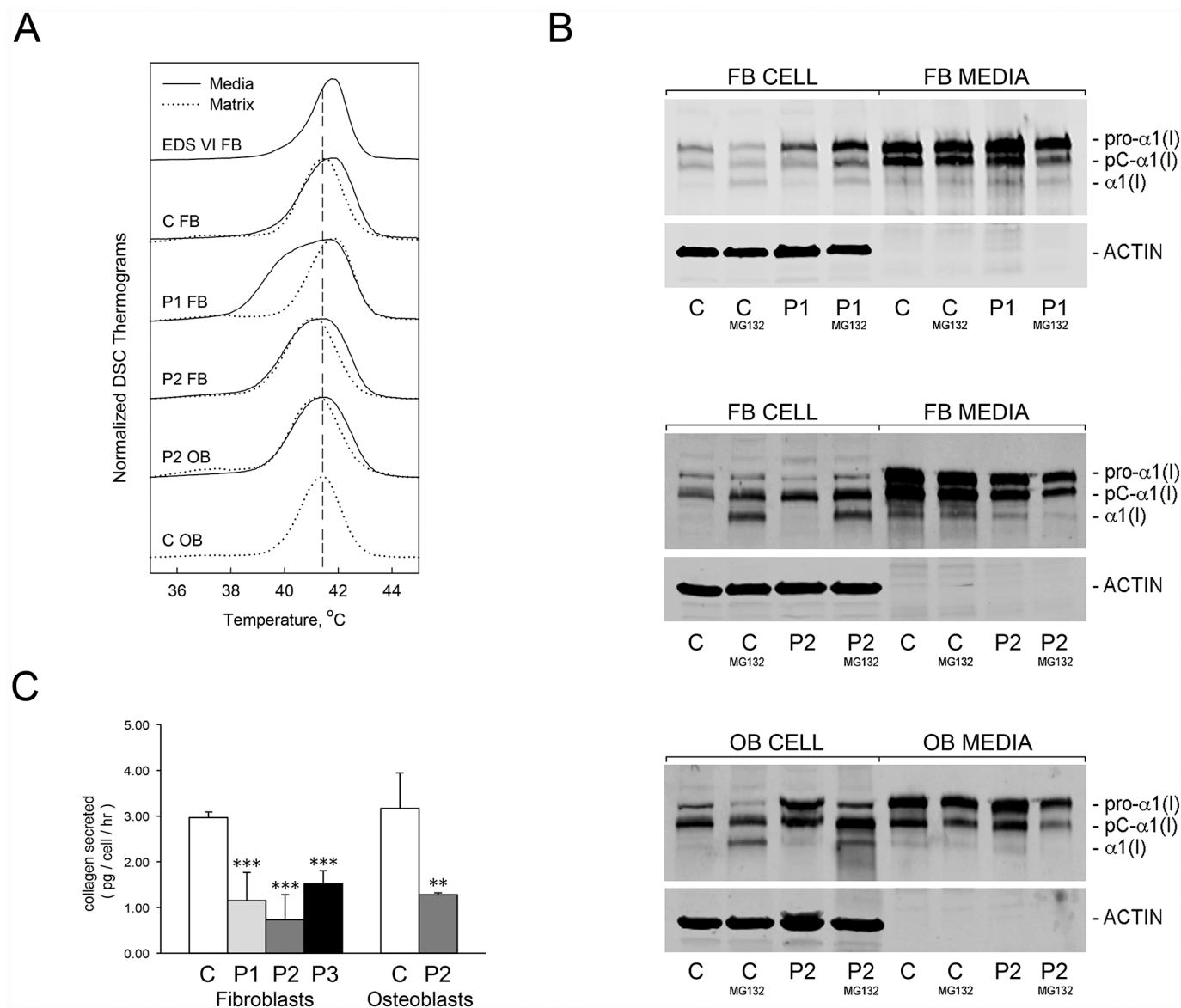
Fig 7. Collagen conformation and secretion are altered by abnormal ER [Ca 2+ ]. (A) Differential scanning calorimetry (DSC) analysis reveals no differences in thermal stability ( T_m ) of type I collagen secreted by control (C, media) and LH1-deficient (EDS VI, media) fibroblast cultures, but a low-stability fraction in proband (P1, P2, media) secreted collagen. Thermal stability of type I collagen extracted from extracellular matrix deposited in culture by control (C, matrix) and proband (P1, P2, matrix) cells is equivalent. (B) Immunoblots of intracellular (cell) and secreted (media) type I collagen from control (C) or proband (P1, P2) fibroblasts (FB) and osteoblasts (OB, P2) cultured in the absence or presence of proteasomal inhibitor (MG132). Retention of type I collagen in proband cells is increased upon treatment. (C) Quantitation of total procollagens in 24 hour conditioned media of control (C) and proband cell cultures. Secretion of procollagens is decreased by more than one-half in proband fibroblasts (P1, P2, P3) and osteoblasts (P2). **, p < 0.01 ; ***, p < 0.001 .
