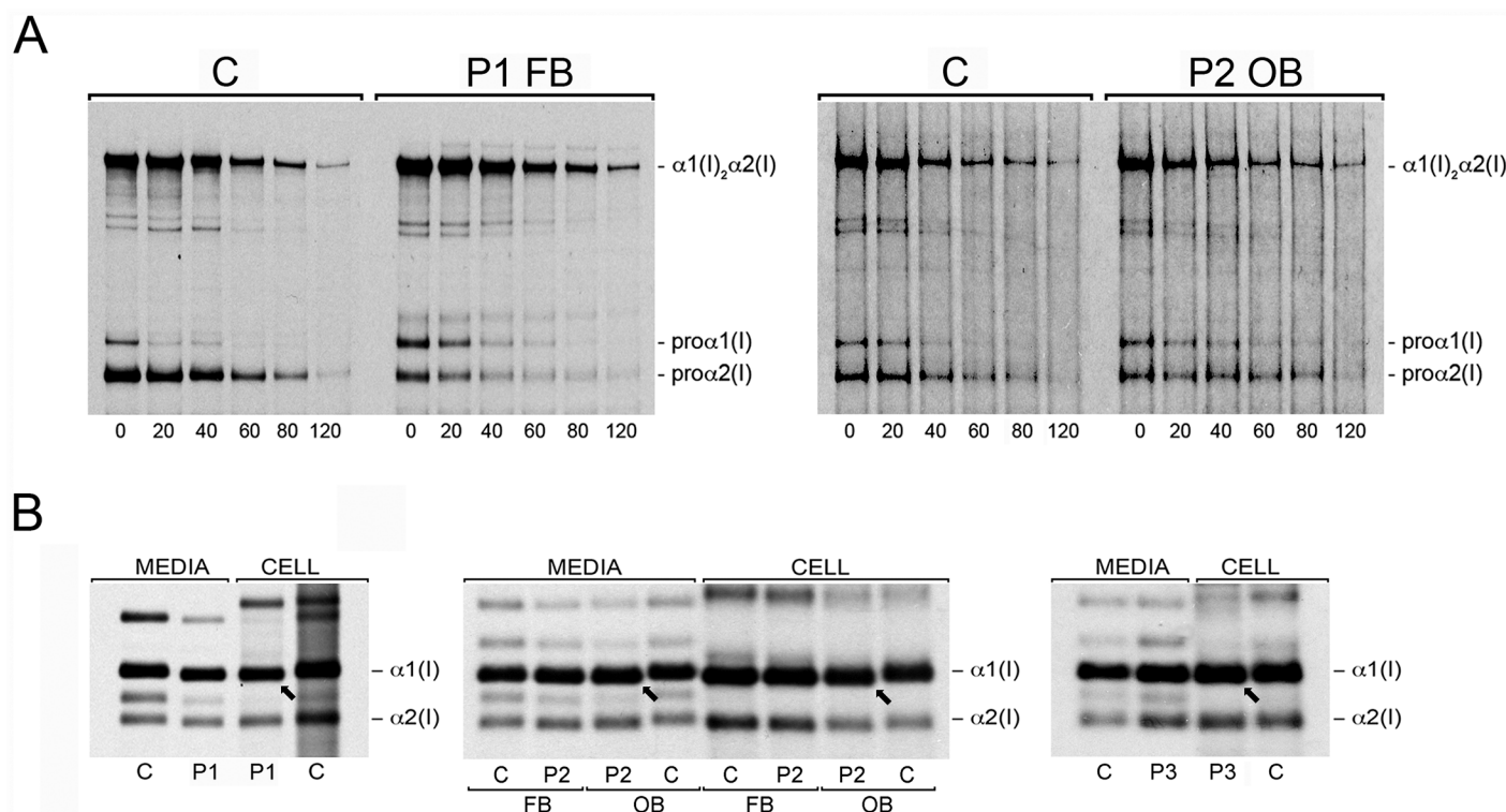
Fig 6. Disruption of ER [\text{Ca}^{2+}] homeostasis dysregulates type I collagen synthesis. (A) Intracellular chain association assay to follow assembly of monomeric pro- \alpha 1(I) and pro- \alpha 2(I) chains into heterotrimeric procollagen molecules, \alpha 1(I)_2\alpha 2(I) , at 20 minute intervals of a pulse-chase analysis. Unincorporated pro- \alpha 1(I) chains are present in proband cells approximately 20 minutes longer in P1 fibroblasts (P1 FB) and P2 (P2 OB) osteoblasts versus normal control fibroblasts and osteoblasts (C). (B) Steady-state cell layer (cell) and secreted (media) collagen from normal control (C) and proband fibroblasts (P1-P3, FB) and osteoblasts (P2, OB) analyzed by SDS-Urea PAGE. Both the \alpha 1(I) and \alpha 2(I) chains of type I collagen from proband cells demonstrate faster electrophoretic migration than normal control type I collagen alpha chains.
