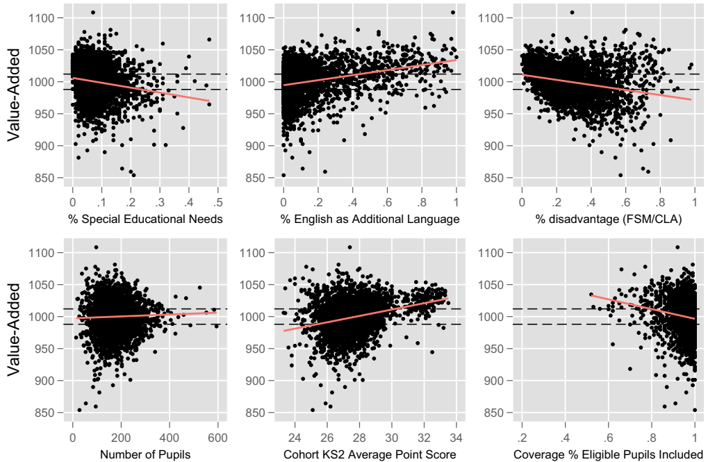
Figure 2. 2014 School KS2-4 Value-Added Scores against selected Contextual Variables at School-Level
