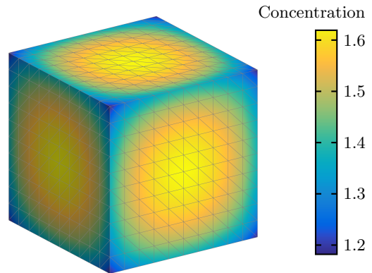
Fig. 7. Surface concentration of a cube with uniform activity \mathcal{A} = 1 and sides of length L = 2 . The double layer constant \lambda = 1/2, 3/7, 7/8 for the faces, edges, and corners respectively.
