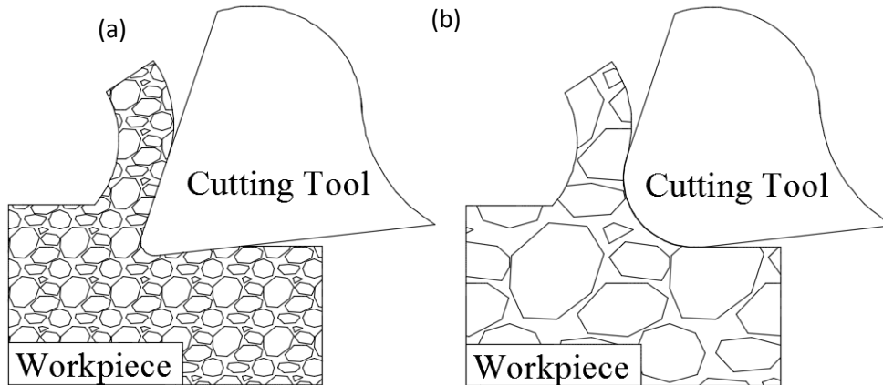
Fig. 1: (a) macro and (b) micro cutting, showing relative dimensions of cutting tool and grain size
