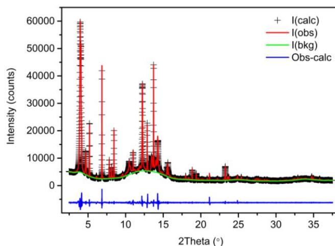
Figure 2: GSAS Rietveld refinement of IPC-2 showing the experimental synchrotron data (red), fitted calculated background (green), calculated model (+) and the observed - calculated difference curve (blue).
