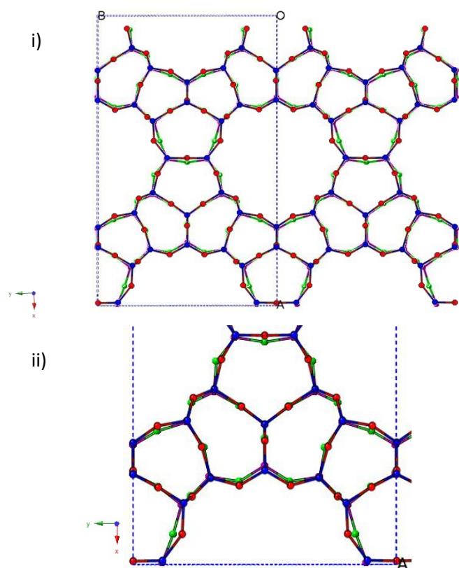
Figure 4: An overlap of IPC-2 (OKO) refinements by PDF (Si atoms in blue, O atoms in red) over Rietveld (Si atoms in purple, O atoms in green) showing the minimal differences between them. i) Shows two unit cells whilst ii) shows a zoomed in section to highlight the finer differences. The unit cells have been rescaled to allow comparison and viewed down the c-axis.
