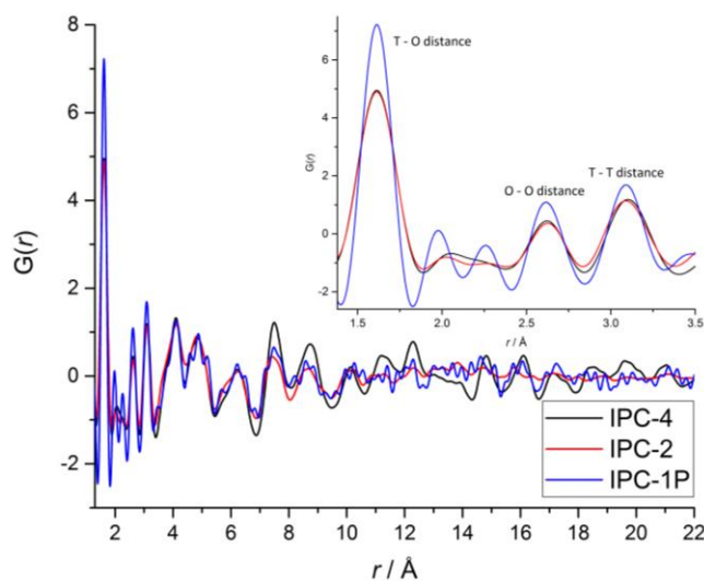
Figure 1: Experimental PDF data of IPC-4 (black line), IPC-2 (red line) and IPC-1P (blue line). The inset labels the structural features immediately discernable without modelling.
