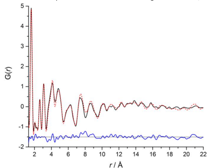
Figure 3: Refinement of the IPC-2 model against PDF data. R_w = 14.5\% . The black solid line is experimental data, the red dashed line is the calculated PDF from the model and the blue line is the difference between the two, offset by -1.5 .
