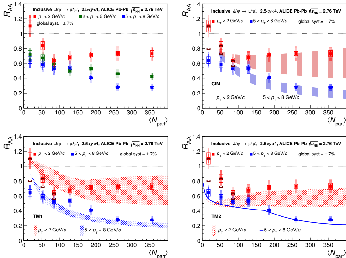
Figure 8. Inclusive J/\psi R_{AA} as a function of the number of participant nucleons measured in Pb–Pb collisions at \sqrt{s_{NN}} = 2.76 TeV for three p_T ranges (0–2, 2–5 and 5–8 GeV/ c ) and comparisons of the lowest and highest p_T range to the transport and to the comover interaction models [13, 60, 63]. The brackets quantify the possible range of variation of the hadronic J/\psi R_{AA} for two extreme hypotheses on the photo-production contamination in the inclusive measurement.
