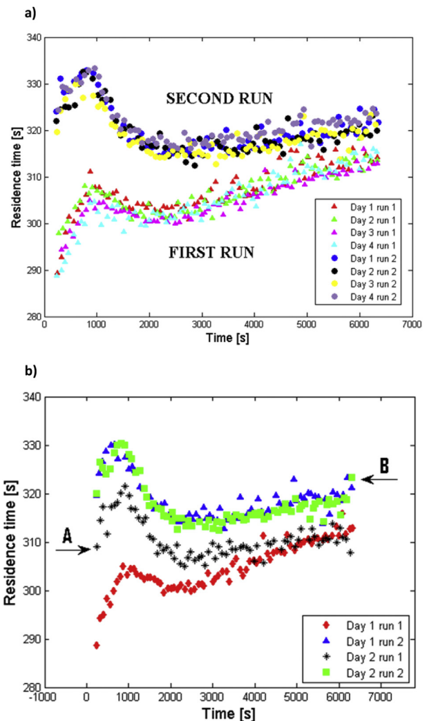
Fig. 7. a) Residence time of barley grains at motor angles of 40^\circ and a motor speed of 600 rpm at four consecutive days (2 runs each day). Cleaning after each day. b) Residence time of barley grains at motor angles of 40^\circ and a motor speed of 600 rpm at two consecutive days (2 runs each day). No cleaning.
