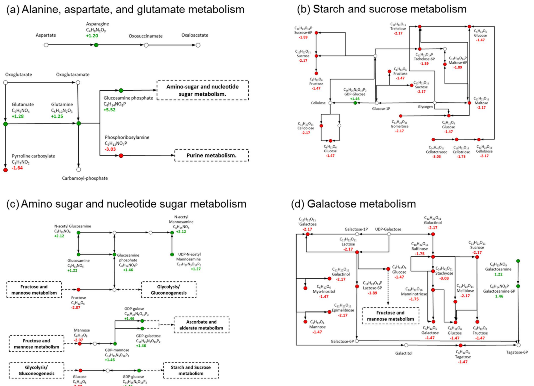
Figure 3. Pathway maps for the alanine, aspartate and glutamate metabolism (a), starch and sucrose metabolism (b), amino sugar and nucleotide sugar metabolism (c), and galactose metabolism (d), adapted from the respective pathways in the KEGG database. Pathways maps are limited to reactions involving putatively annotated compound names associated with significantly increasing (green ●) or decreasing (red ●) m/z peaks in response to the short-day conditions. The positive or negative fold change of the most stable detected m/z ion form is displayed for each putative compound name. Compounds that were not detected, but which are known to be involved in these reaction pathways, are also included (○). Solid black lines represent interactions between pathway components. Dashed lines are included when a particular metabolite is also included in another KEGG pathway.
