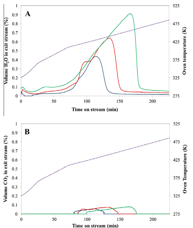
Fig. 2. Evolution of (A) H 2 O and (B) CO 2 during the initial CuO/ZnO/Al 2 O 3 reduction step under 2% H 2 /N 2 at 10 bar. (—) denotes 125 mg bed, (—) 250 mg bed, (—) 500 mg bed and (---) oven temperature (K).
