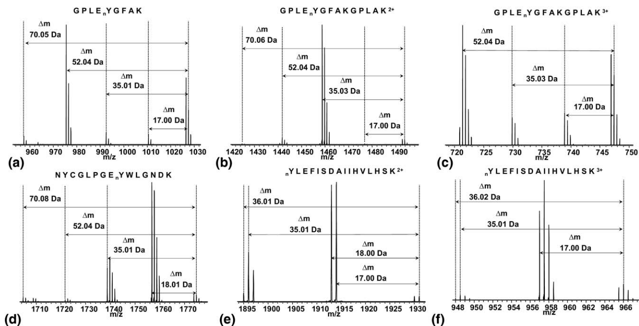
Figure 3. Expanded m/z regions of ECD mass spectra showing peaks corresponding to neutral losses from the charge-reduced cation radical for precursor ions: (a) [\text{GPLEnYGFYAK} + 2\text{H}]^{2+} , (b) [\text{GPLEnYGFYAKGPLAK} + 2\text{H}]^{2+} , (c) [\text{GPLEnYGFYAKGPLAK} + 3\text{H}]^{3+} , (d) [\text{NYCGLPGE nYWLGN DK} + 2\text{H}]^{2+} , (e) [\text{nYLEFISDAIIHVLH SK} + 2\text{H}]^{2+} , and (f) [\text{nYLEFISDAIIHVLH SK} + 3\text{H}]^{3+} . Mass shifts ( \Delta m ) from the mass of the charge-reduced [\text{M} + 2\text{H}]^{+} and [\text{M} + 3\text{H}]^{2+} ions for doubly-charged and triply-charged precursor ions, respectively, are indicated.
