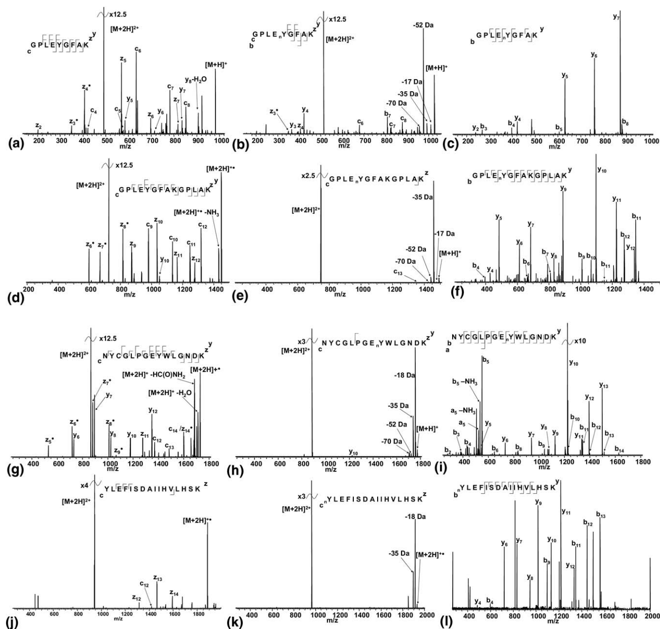
Figure 1. MS/MS spectra of doubly-charged peptides: (a) ECD of [GPLEYGFAG + 2H]^{2+} ions; (b) ECD of [GPLEnYGFAG + 2H]^{2+} ions; (c) CID of [GPLEnYGFAG + 2H]^{2+} ions; (d) ECD of [GPLEYGFAGPLAK + 2H]^{2+} ions; (e) ECD of [GPLEnYGFAGPLAK + 2H]^{2+} ions; (f) CID of [GPLEnYGFAGPLAK + 2H]^{2+} ions; (g) ECD of [NYCGLPGEYWLGN DK + 2H]^{2+} ions; (h) ECD of [NYCGLPGEYWLGN DK + 2H]^{2+} ions; (i) CID of [NYCGLPGEYWLGN DK + 2H]^{2+} ions; (j) ECD of [YLEFISDAIIHVLH SK + 2H]^{2+} ions; (k) ECD of [nYLEFISDAIIHVLH SK + 2H]^{2+} ions; (l) CID of [nYLEFISDAIIHVLH SK + 2H]^{2+} ions. nY denotes 3-nitrotyrosine.
