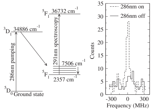
FIG. 2. Optical pumping scheme used for Nb. The effect of the 286.6 nm pumping light on the 290.9 nm fluorescence signal, the F = 9 \rightarrow F = 9 component of ^{90}\text{Nb} , is shown.
