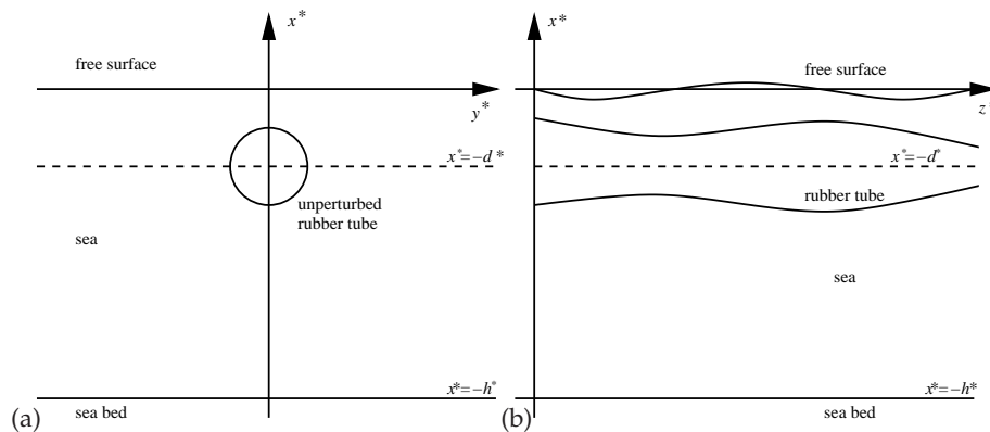
Figure 1. Two schematics of the distensible tube in the sea showing cross-sections (a) from the front and (b) from the side, where the x^* -axis is vertical, the y^* -axis is horizontal and the z^* -axis is parallel to the axis of the unperturbed tube.
