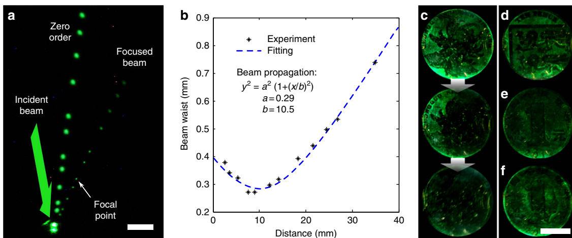
Figure 5 | Active optical elements and 3D holograms. (a) A reconfigurable lens with a focal distance of 10 mm reconstructed with multiple images of the beam path (scale bar, 5 mm). (b) Beam waist measured along the path corresponding to the reconfigurable lens. (c) A 3D hologram of a coin recorded with interference of beams and its erasing process (scale bar, 1 cm). (d,e) Two different coins recorded after an erasing process. (f) Two coins superposed without an intermediate erasing process.
