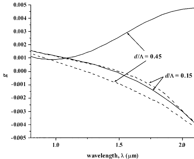
Figure 5 Total normalized GVD obtained by analytically evaluating the sum of material and waveguide dispersion (dashed lines) and by numerical differentiation (solid lines)
