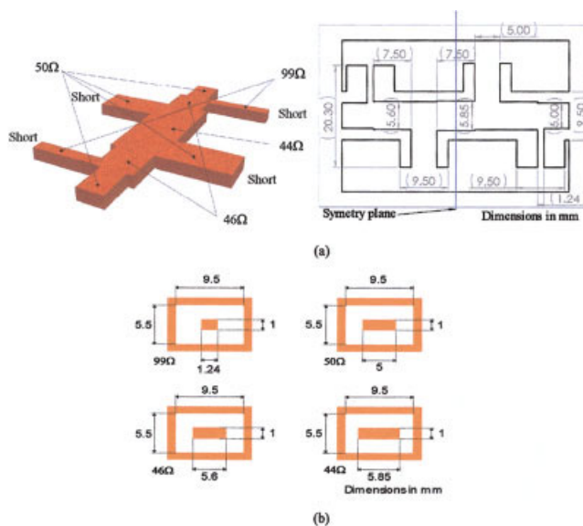
Figure 2 Suspended coaxial transmission line supported by stubs: (a) center conductor only and the dimensions of layer 3; (b) cross section of the different impedance coaxial transmission-line sections. [Color figure can be viewed in the online issue, which is available at www.interscience.wiley.com .]
