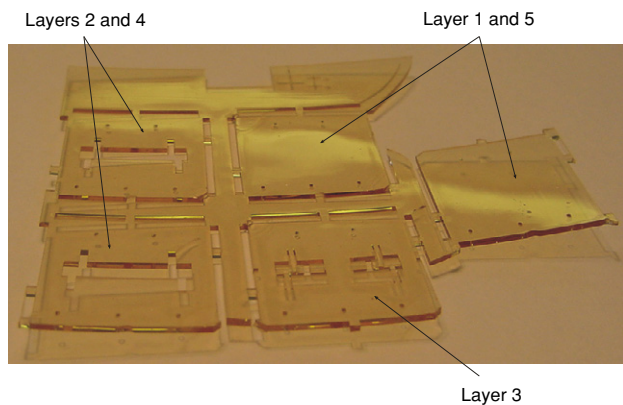
Figure 8. 700 \mu\text{m} thick layers of the Ka-band filter made of SU-8.
