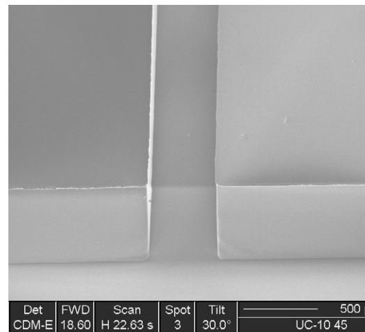
Figure 6. An SU-8 layer of 700 \mu\text{m} thickness, fabricated for the filter.
