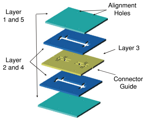
Figure 1. Coaxial assembly of the Ka-band dual mode filter.
