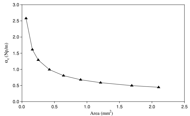
Figure 4. Attenuation constant for an air filled, 50 \Omega square coaxial transmission lines versus the area of the cross-section used.
