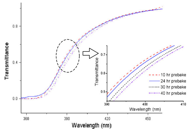
Figure 5. UV transmission spectra of unexposed ultra-thick SU-8 layers coated on glass.
