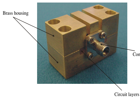
Figure 9. Photograph of a complete layered coaxial device.
