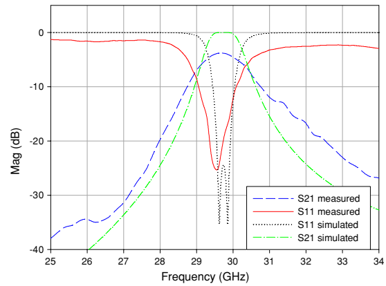
Figure 3. Response of the prototype filter.
