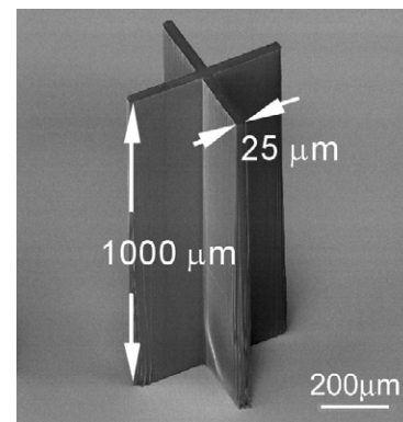
Figure 7. An SEM image of a high aspect ratio cross.
