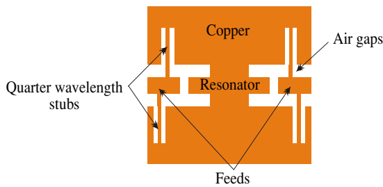
Figure 2. Centre conductor of the filter.
