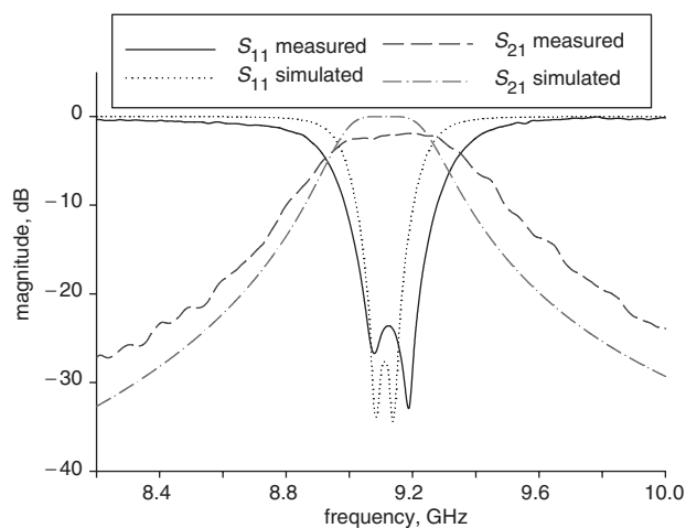
Fig. 9 Response of the dual-mode X-band filter
