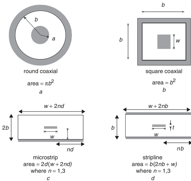
Fig. 3 Various different types of transmission line
