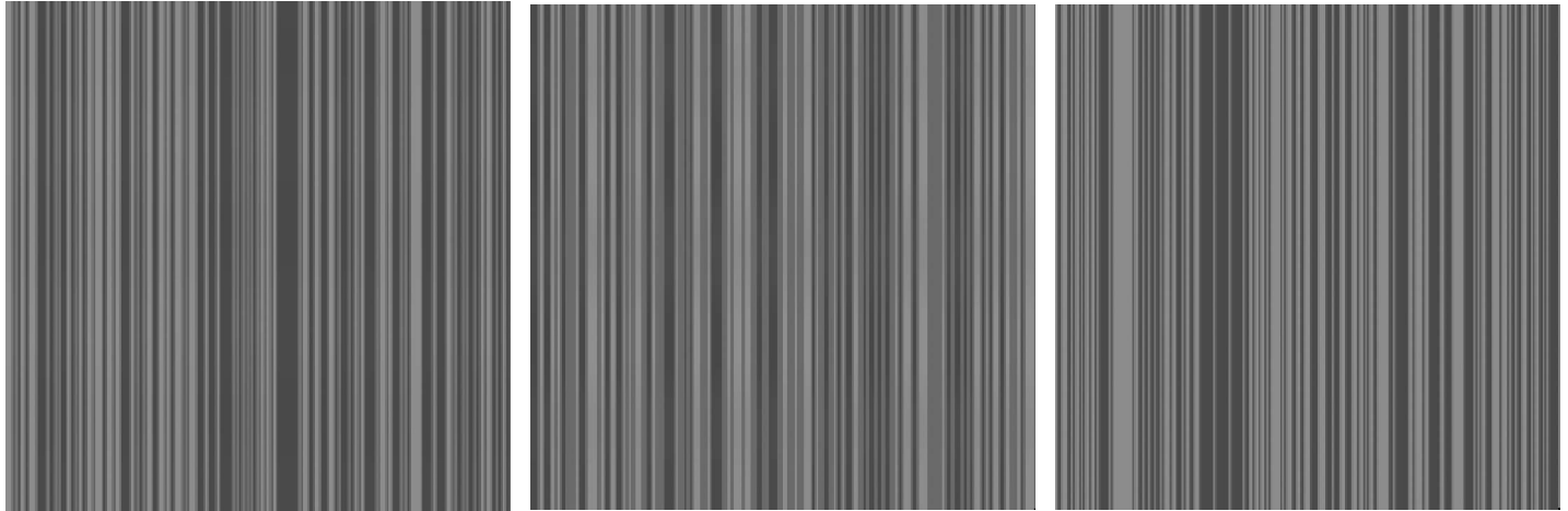
Movies 4–6. Sample test sequences for Experiment 3 . Test sequences comprised two counterphasing components that are fully balanced in these examples so as to produce “flicker” rather than motion. Left panel, Movie 4, LM; middle panel, Movie 5, CM; right panel, Movie 6, OM. Test sequences lasted for 1 s. As static images, only the first unmodulated frame is shown. The reader is referred to Movies 1–3 , which better illustrate our cues in a static presentation.
