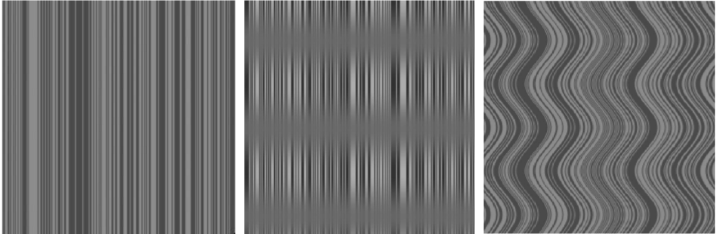
Movies 1–3. Sample stimuli: Movies 1–3 show motion sequences for the three cues used in this study. Left panel, Movie 1, LM; middle panel, Movie 2, CM; right panel, Movie 3, OM. Such sequences were used in Experiments 1 and 2 (duration = 1 s) and as the adapters in Experiment 3 (for duration see text). As static images, Movies 1–3 demonstrate the appearance of a single frame in our motion sequences. See text for details.
