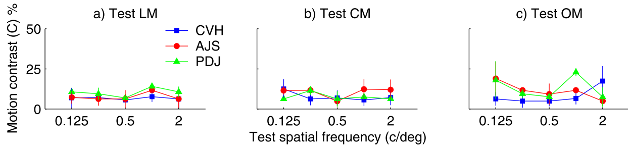
Figure 4. Sensitivity to motion contrast in test. Circles, squares, and triangles represent data for observers A.J.S., C.V.H., and P.D.J., respectively. Error bars are as described in Figure 1.
