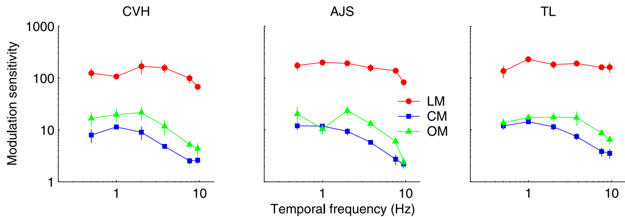
Figure 2. Sensitivity as a function of temporal frequency; details are as described in Figure 1.
