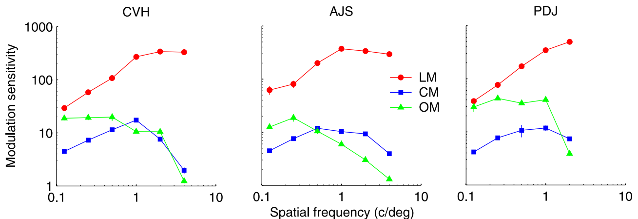
Figure 1. Sensitivity as a function of spatial frequency; circles, squares, and triangles show sensitivity to LM, CM, and OM, respectively. Error bars show 95% confidence intervals estimated from 5,000 iterations of a nonparametric bootstrap procedure.
