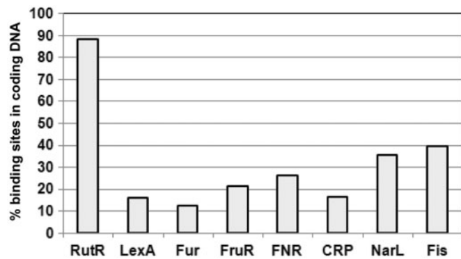
Figure 4. Distribution of sites for global DNA-binding proteins between coding and non-coding DNA in the E. coli chromosome. Using equally stringent search conditions for each factor, we screened the E. coli MG1655 genome for DNA sequences that resembled the DNA-binding sites of RutR, LexA, Fur, FruR, FNR, CRP, NarL and Fis. The results show that, while predicted high-affinity-binding sites for most factors are found in non-coding DNA, most sequences resembling the RutR-binding site were found in coding DNA.
