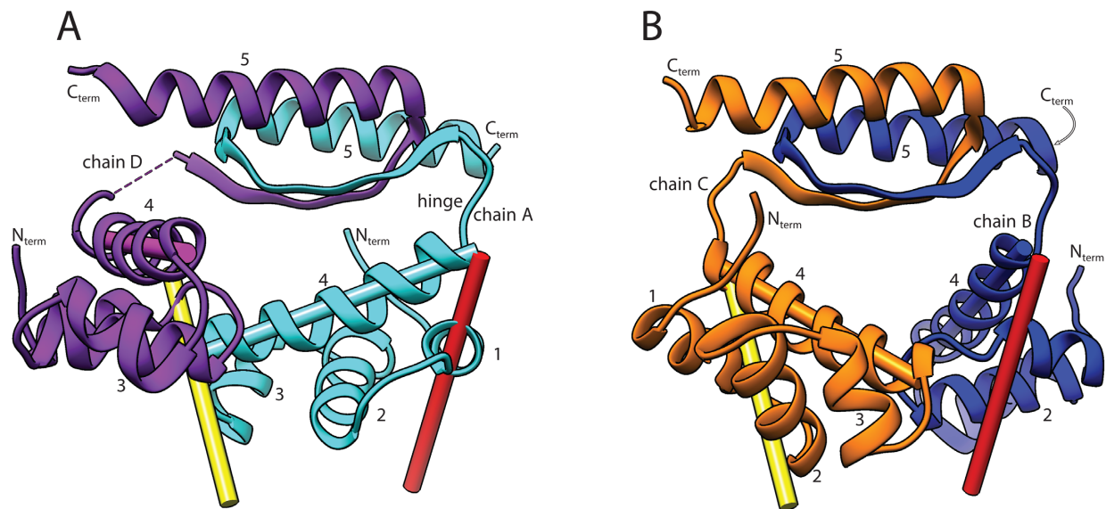
Figure 1. Ribbon diagrams of the X-ray structure of the free KorA dimers (PDB ID: 5CKT). Each subunit is labelled chain A–D at the corresponding flexible hinge region and at the N- and C-termini, while the helices are numbered 1–5 in the N to C direction. The recognition helices of the DNA-binding helix–turn–helix motifs are highlighted with a cylinder of the appropriate colour. The red and yellow cylinders indicate the approximate position of the corresponding helices in the KorA–DNA complex (PDB ID: 5CM3). (A) KorA ribbon diagram for Subunits A (cyan) and D (purple). The hinge of chain A is labelled. There is no electron density for the hinge region (residues 65–69 inclusive) in Subunit D, indicating disorder. (B) KorA ribbon diagram for Subunits B (blue) and C (orange).
