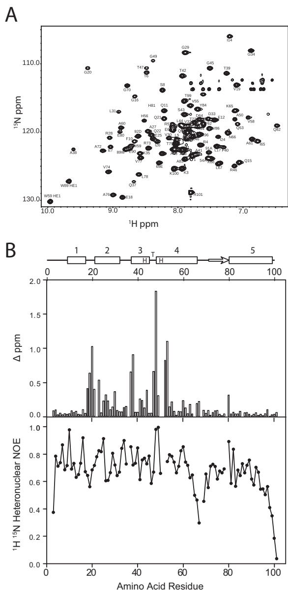
Figure 4. NMR data of KorA bound to a 20-bp oligonucleotide containing the \text{O}_A consensus sequence. (A) ^{15}\text{N} - ^1\text{H} HSQC of KorA- \text{O}_A at 308K recorded at 600 MHz. The peaks are labelled with the amino acid assignments of their NH group, the two peaks at \sim 10 ppm are from the indole NH groups of the two tryptophan residues. (B) Top: schematic secondary structure of KorA, the boxes show the \alpha -helices, which are numbered and the arrow shows the \beta -strand. HTH indicates the position of the helix-turn-helix motif. Centre: combined ^{15}\text{N} and ^1\text{H} chemical shift differences between free protein and DNA-bound amide resonances of KorA. Bottom: ratio of peak intensities of ^{15}\text{N} - ^1\text{H} HSQC spectra of the KorA- \text{O}_A complex taken without and with proton saturation of 2.9 s, giving heteronuclear ^{15}\text{N} - ^1\text{H} NOE.
