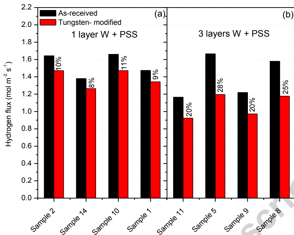
Figure 4: Comparison of the room temperature hydrogen flux for selected samples before and after the modification with (a) 1 layer and (b) 3 layers of tungsten powder.
