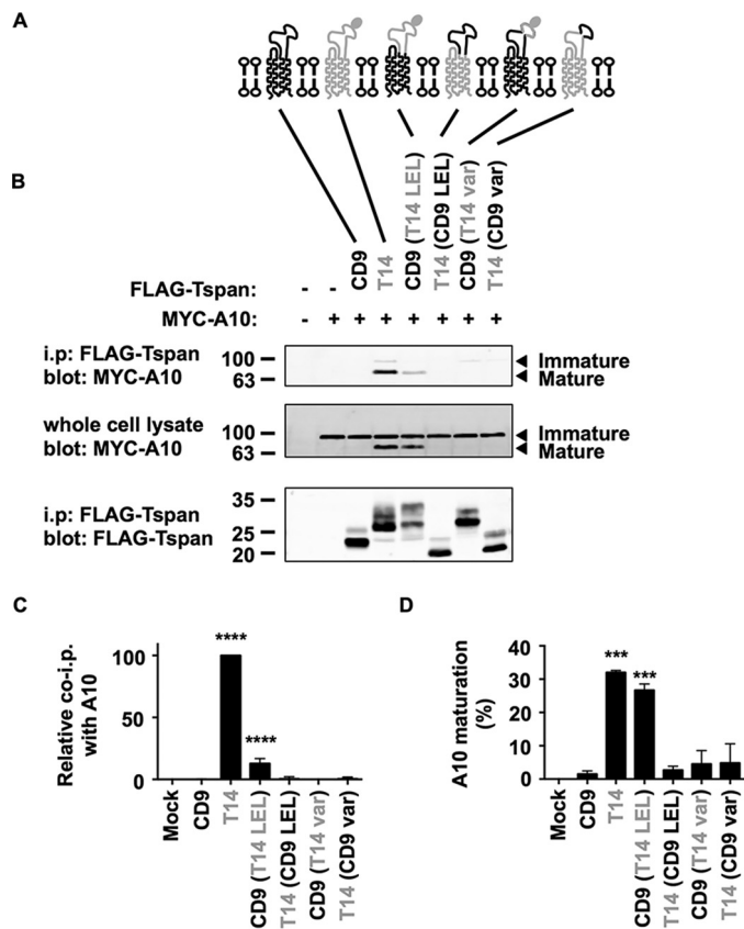
FIGURE 2. The large extracellular loop (LEL) of Tspan14 is the region that interacts with ADAM10 and is required for ADAM10 maturation. A, schematic of Tspan14 and CD9 chimeras. The large extracellular loop (LEL) and variable (var) region of CD9 (black) and Tspan14 (gray) were interchanged; the N-linked glycosylation site of Tspan14 is indicated by a filled oval. B, HEK-293T cells were mock transfected (–) or transfected with expression constructs containing the FLAG-tagged human tetraspanin chimeras with Myc-tagged human ADAM10 (+). Cell lysates were produced using 1% digitonin lysis buffer and immunoprecipitated with an anti-FLAG antibody. Immunoprecipitated proteins were blotted with anti-Myc tag antibody ( top panel ) or anti-FLAG antibody ( lower panel ). Whole cell lysates were probed with the anti-Myc tag antibody ( middle panel ). Data are representative of three independent experiments. C, quantitation of immunoprecipitated ADAM10. Data in panel B ( upper panel ) were quantitated using the Odyssey Infrared Imaging System (LI-COR), and the amount of ADAM10 immunoprecipitated was shown relative to immunoprecipitated Tspan14, which was arbitrarily set at 100. Data were normalized by log transformation and statistically analyzed using a one-way ANOVA with a Dunnett's multiple comparison test compared with the mock (****, p < 0.0001 ). Error bars represent standard error of the mean from three experiments. D, data in panel B ( middle panel ) were quantitated, the percentage of mature ADAM10 calculated, and the data log transformed and statistically analyzed as described for panel C (***, p < 0.001 ).
