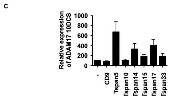
FIGURE 6. All TspanC8s interact with the region of ADAM10 comprising the disintegrin (D), cysteine-rich domain (C), and stalk (S). A, HEK-293T cells were transfected with expression constructs for the HA-tagged mouse ADAM17 10DCS chimera and FLAG-tagged mouse TspanC8s, CD9 or negative control (–). Lysates were extracted in 1% digitonin lysis buffer and proteins immunoprecipitated with an anti-FLAG antibody. Immunoprecipitates were blotted with anti-HA tag antibody (top panel) or anti-FLAG antibody (lower panel). Whole cell lysates were probed with the anti-HA tag antibody (middle panel). B, data in panel A (upper panel) were quantitated, and the amount of ADAM17 10DCS immunoprecipitated was normalized for the amount in the whole cell lysate. Data are shown relative to immunoprecipitated Tspan14, which was arbitrarily set at 100. Data were normalized by log transformation and statistically analyzed using a one-way ANOVA with a Dunnett's multiple comparison test compared with the mock. All TspanC8s bound significantly to ADAM17 10DCS ( p < 0.0001 ). Error bars represent standard error of the mean from three experiments. C, ADAM17 10DCS whole cell lysate data in panel A were quantitated, and the amount of ADAM17 10DCS expressed was normalized to the expression in the first lane, which was arbitrarily set at 100. Error bars represent standard error of the mean from three experiments.
