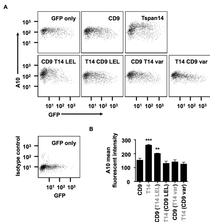
FIGURE 3. The large extracellular loop (LEL) of Tspan14 is critical for its ability to increase ADAM10 cell surface accumulation. A, HeLa cells were transfected with the indicated Tspan14-CD9 chimeras (see Fig. 2A) and GFP to identify transfected cells. Cells were stained with an APC-conjugated ADAM10 antibody and analyzed by flow cytometry. Dot plots are representative of three independent experiments. The bottom left panel shows isotype control staining. B, average geometric mean fluorescent intensities for ADAM10 staining, gated on live and GFP-positive cells, were compared statistically using a one-way ANOVA with a Dunnett's multiple comparison test, compared with the CD9 control (***, p < 0.001 ; **, p < 0.01 ). Error bars represent standard error of the mean from three experiments.
