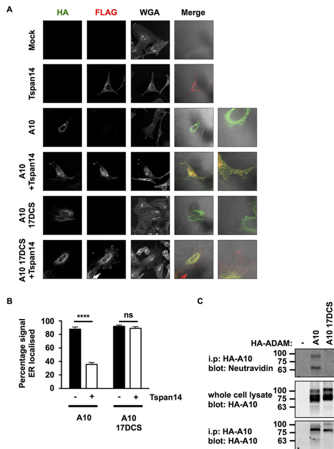
FIGURE 7. The disintegrin (D), cysteine-rich (C), and stalk (S) regions of ADAM10 are essential for Tspan14-mediated exit from the ER. A, HEK293T cells were transfected with combinations of FLAG-tagged Tspan14 and HA-tagged mouse ADAM10 wild-type or ADAM10 17DCS. Cells were fixed and stained with an anti-HA antibody (green), an anti-FLAG antibody (red) and WGA to visualize the plasma membrane and internal cellular structures by confocal microscopy. B, HEK293T cells were transfected and stained as in panel A except an anti-calnexin antibody was used instead of WGA to define the limits of the ER (images not shown). The HA signal was quantitated across the whole cell and within the mask of the calnexin staining, and presented as a percentage of HA-ADAM10 or HA-ADAM10 17DCS signal localized in the ER. Data are representative of three independent experiments and at least 15 fields of view. A two-way ANOVA statistical analysis was performed with a Bonferroni's multiple comparisons test ( ns , non-significant, **** , p < 0.0001 ). C, HEK-293T cells were mock transfected (–), or transfected with HA-tagged mouse ADAM10 wild-type or ADAM10 17DCS. Cells were surface biotinylated, lysed, and immunoprecipitated with an anti-HA antibody. Immunoprecipitates were stained with neutravidin (top panel) or an anti-HA antibody (bottom panel). Whole cell lysates were stained with an anti-HA antibody (middle panel).
