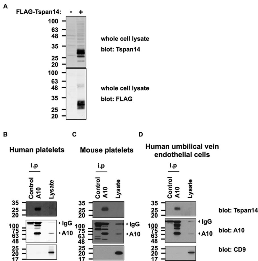
FIGURE 1. Endogenous ADAM10 and Tspan14 interact in platelets and primary endothelial cells. A, HEK-293T cells were mock transfected (–) or transfected with a FLAG-tagged human Tspan14 expression construct (+). The cells were lysed in 1% Triton X-100 lysis buffer and subjected to anti-Tspan14 (top panel) and anti-FLAG (lower panel) Western blotting. The Tspan14 antibody was raised in goat against a C-terminal cytoplasmic peptide, in collaboration with Everest Biotech. B, washed human platelets; C, washed mouse platelets and D, human umbilical vein endothelial cells were lysed in 1% digitonin lysis buffer, and proteins were immunoprecipitated with an antibody against ADAM10 or an isotype-matched control. Precipitates were then run on non-reducing gels, Western blotted, and probed with Tspan14 (top panels), ADAM10 (middle panels), and CD9 (lower panels) antibodies. Arrows indicate the positions of the predominant mature form of ADAM10 (A10) and the signal from the immunoprecipitating antibodies (IgG).
