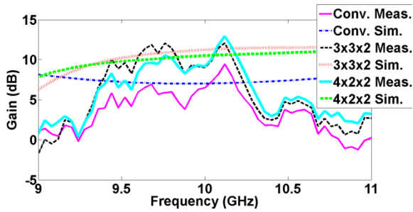
Fig.12. Comparison between the measured and the simulated gains of the proposed antenna with and with CSRRs/TWs periodic structure of different sizes and fixed separation h_s of 10 mm between the patch and the CSRRs/TWs periodic structure.
