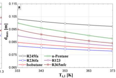
Fig. 7. Variation of T_{t,1} for 6 fluids
