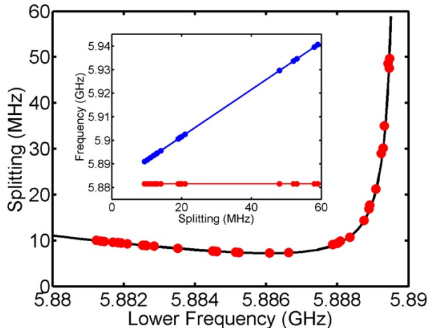
FIG. 4. Splitting between the upper and lower frequency branches of sample 4 as a function of the frequency of the lower branch above the tuning disc having the lower untuned resonant frequency. Lowering the disc decreases the resonator inductance and takes the resonators through the middle of the avoided crossing. The solid lines are from the simulations, where we have set the inductance per unit length to the theoretical value 25 4 \times 10^{-7} H/m and capacitance per unit length to 1.8 \times 10^{-10} F/m. The inset shows the upper and lower resonant peaks as a function of f_{\text{splitting}} when the tuning disc was sited above the resonator with the higher frequency using the same fitting parameters. A 50 MHz shift of the tuned resonator is easily obtained while the untuned resonator is essentially unaffected.
