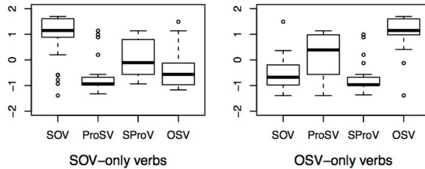
Figure 7: Experiment 2. Box plots of grammaticality ratings (z-scores) for four sentence types (SOV, ProSV, SProV and OSV) with verbs that had been presented only in SOV during exposure (left) or only in OSV during exposure (right). SOV and OSV were functionally equivalent.
