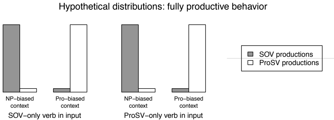
Figure 3b: Hypothetical proportions of SOV and ProSV productions predicted by full productivity, in which productions depend only on the information structure of the two constructions witnessed, and not on how the verbs were presented in the input.
