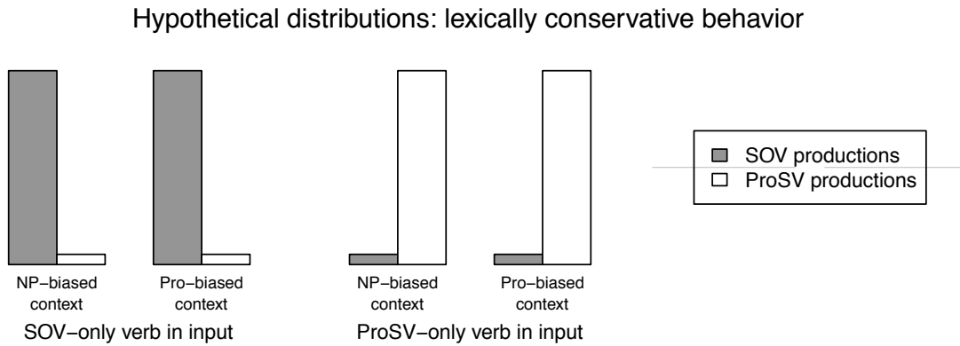
Figure 3a: Hypothetical proportions of SOV and ProSV productions predicted by lexical conservatism in which productions depend only on whether verbs were SOV or ProSV in the input.
