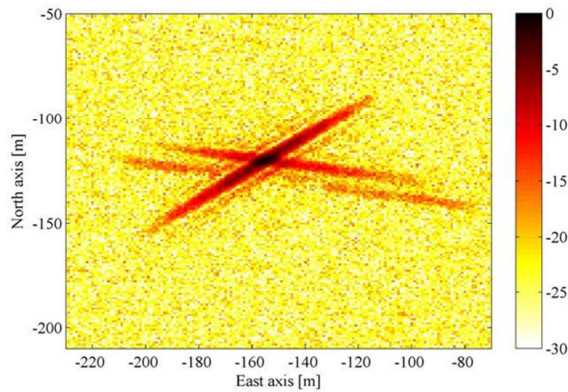
Fig. 10. Residual MSAR image after the first iteration of the multistatic CLEAN.
