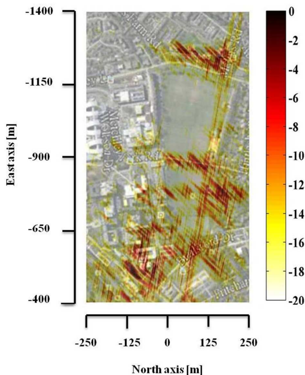
Fig. 16. Experimental MSAR image
