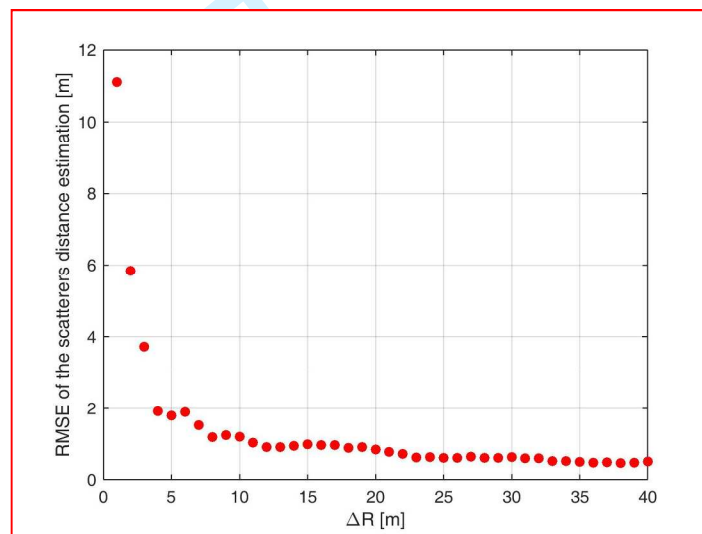
Fig. 7. Root Mean Square Error of the scatterers distance estimation in the multistatic case.
