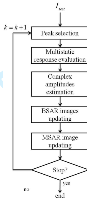
Fig. 4. Joint bistatic/multistatic SAR CLEAN for MSAR images processing scheme.
