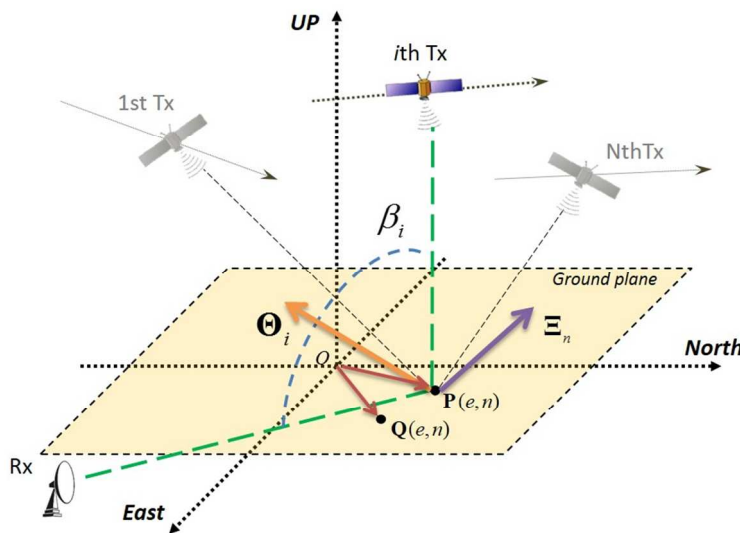
Fig. 1. GNSS-based SAR topology.
