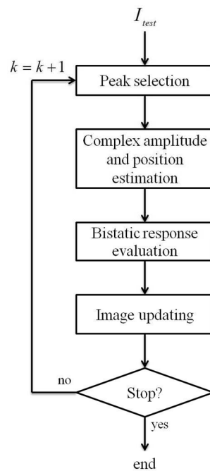
Fig. 3. Coherent CLEAN for bistatic images processing scheme.
