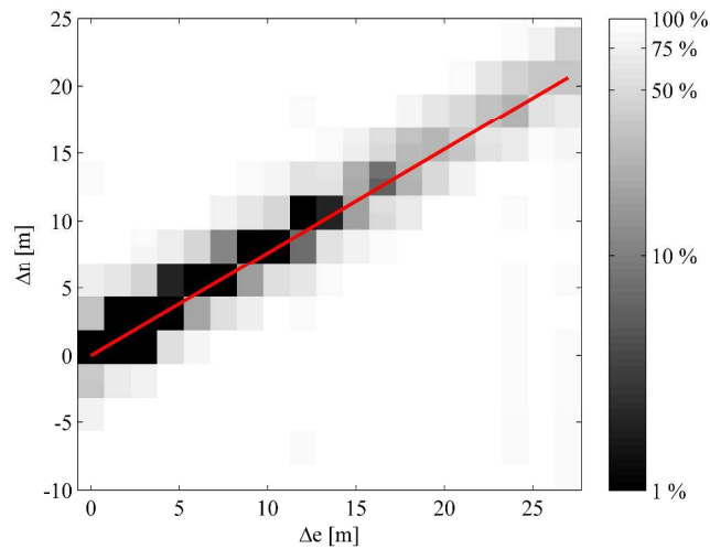
Fig. 5. Probability of correct feature extraction over the (\Delta e, \Delta n) plane for the bistatic case ( \Delta p = 10 m, \Delta A = 0.5 ).
