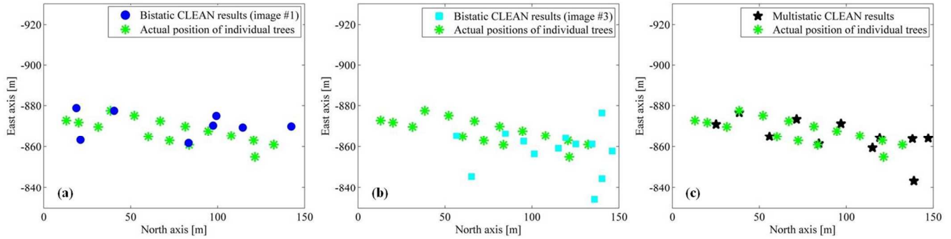
Fig. 18. Comparison actual position of individual trees and dominant scatterers extracted by the CLEAN algorithms.
