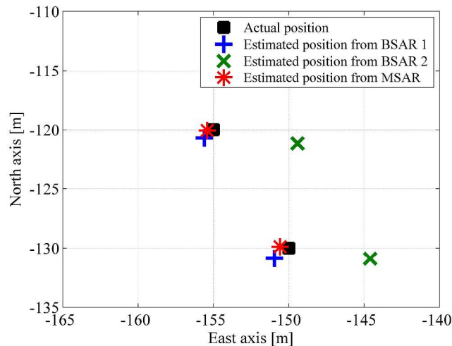
Fig. 9. Comparison actual vs estimated position by the bistatic and multistatic CLEAN.
