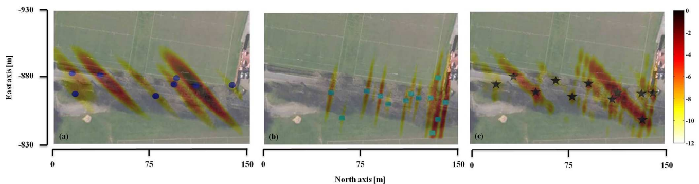
Fig. 17. Tree-lines at the middle-range – a) BSAR #1, b) BSAR #3, c) MSAR.
