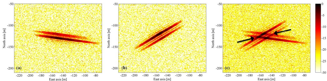
Fig. 8 Emulated GNSS-based SAR images of two point scatterers – a) BSAR image 1, b) BSAR image 2, c) MSAR image.
