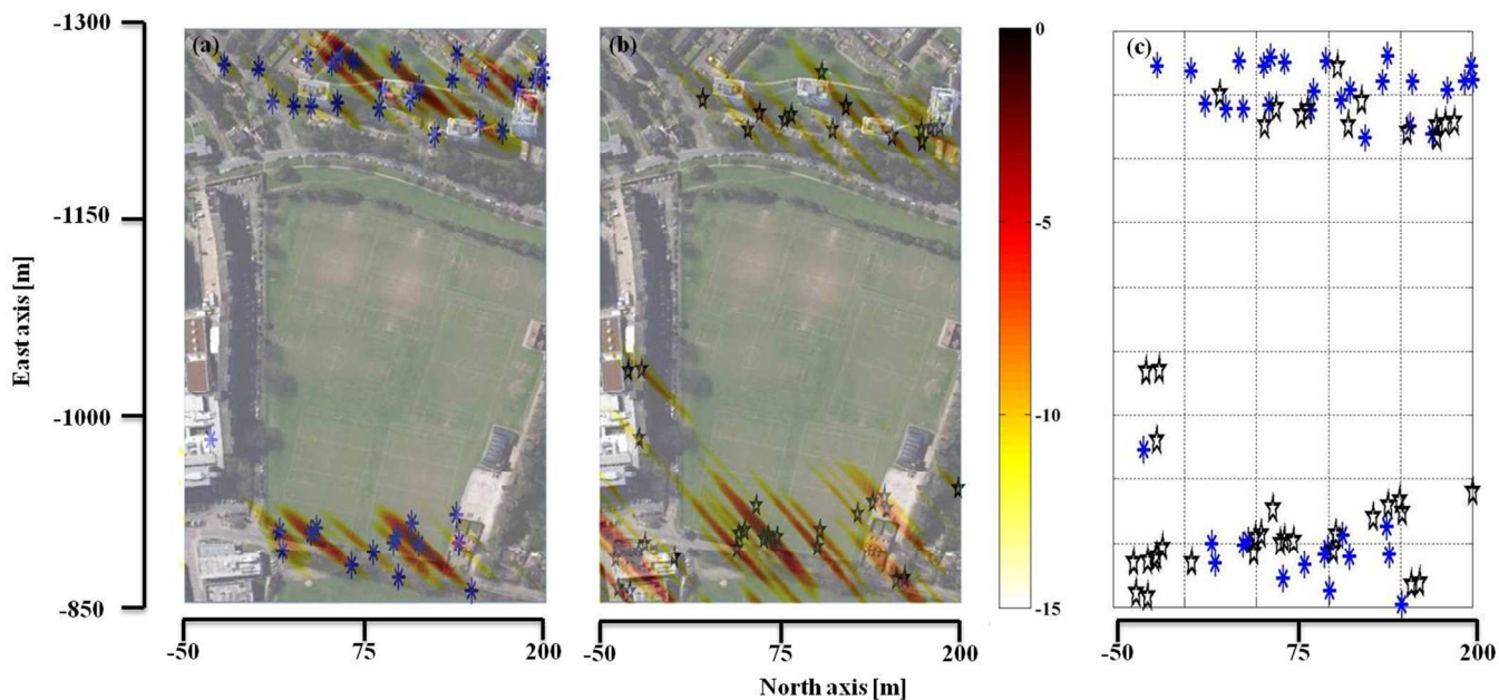
Fig. 15 Multi-perspective analysis – a) BSAR #1, b) BSAR #2, c) scatterers map.
