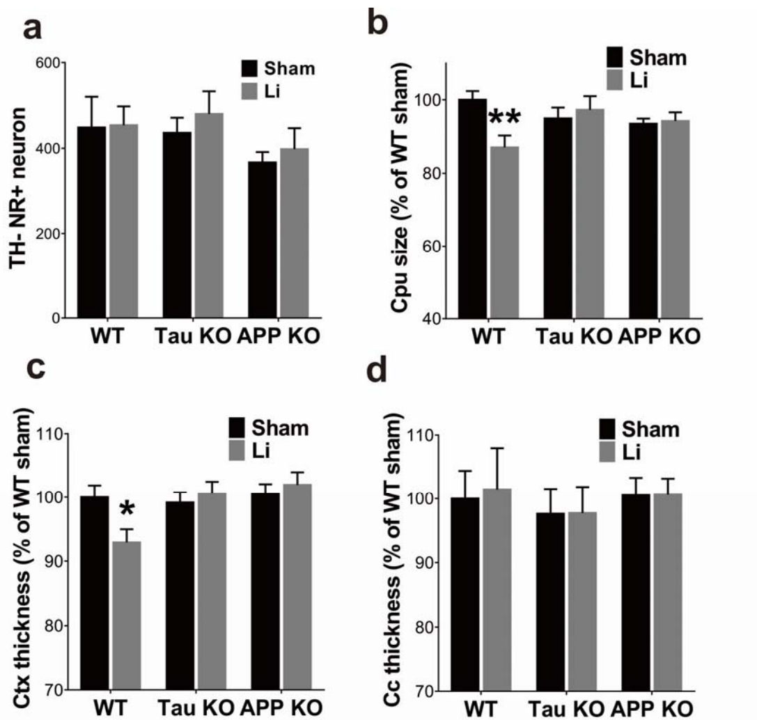
Supplementary Figure 14. Other neuroanatomical changes induced by Li. a) No significant reduction was found in TH-negative, Neutral Red-positive neurons in the SN of Li-treated mice. b-c) Li treatment reduced CPU size [ b ; two-way ANOVA with post-hoc Dunnett's test: no genotype ( p=0.606 ) or treatment ( p=0.153 ) effects, but interaction ( p=0.017 )] and cortical thickness [ c ; genotype ( p=0.041 ) and interaction ( p=0.043 ) effects, but no treatment ( p=0.371 ) effect] in wild type mice, but the effect was abolished by loss of tau or APP. d) No change in corpus callosum thickness was detected in all three mouse strains. Means \pm SEM are shown, n=9-11 per treatment group. * p<0.05 , ** p<0.01 .
