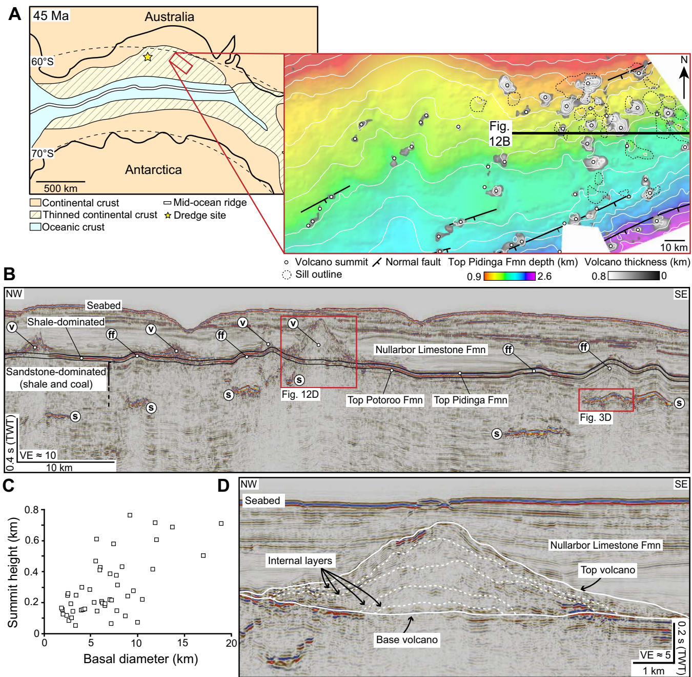
Figure 12. (A) Paleogeographic reconstruction (modified from Espurt et al., 2009) documenting the regional structure immediately prior to the emplacement of a suite of volcanoes mapped in the Ceduna subbasin (inset) (modified from Magee et al., 2013b). (B) Seismic section delimiting high-amplitude reflections (s—sills), forced folds (ff), and volcanoes (v) (modified from Jackson et al., 2013). Fmn—formation; TWT—two-way traveltime; VE—vertical exaggeration. (C) Plot of volcano basal diameter against summit height (Magee et al., 2013b). (D) Internal reflections within a volcano that are inferred to relate to discrete tuff layers and/or lava flows.
