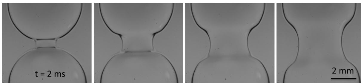
Fig. 6. Images of the coalescing drops of aqueous solution of SLES taken every 2 ms in surrounding 9.3 Pa s silicone oil.
