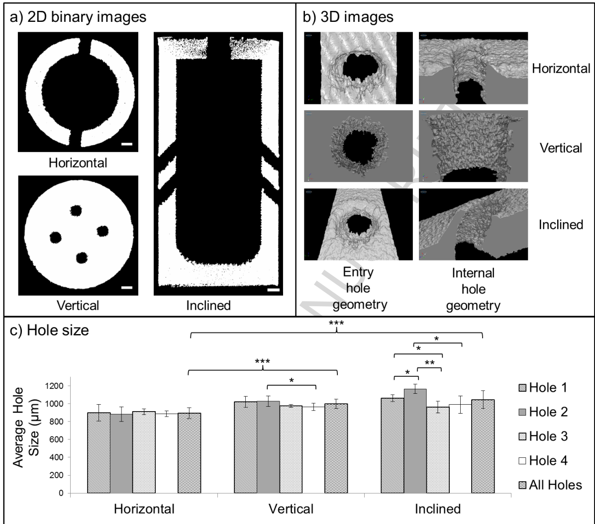
Figure 4: Microstructure of SLM implants a) 2D binary images of hole geometries (scale bars 1 mm), b) 3D reconstruction of hole ROI, and c) measurements of hole size presented as mean \pm standard deviation ( n=4 for individual hole measurements and n=16 for all hole measurements). * p<0.05 , ** p<0.01 , *** p<0.001
