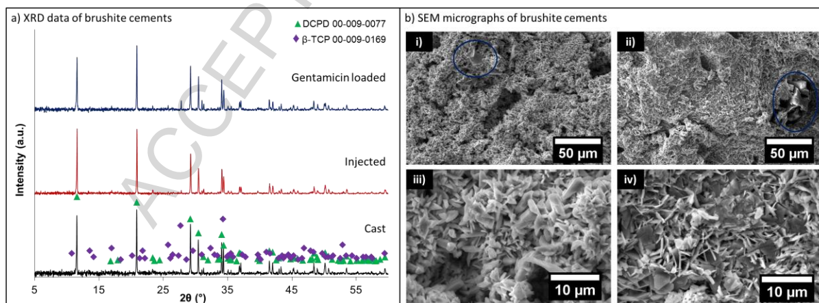
Figure 2: Characterisation of brushite cement samples a) XRD data of cast, injected, and gentamicin loaded cements illustrating matching to DCPD ( \blacktriangle 00-009-0077) and \beta -TCP ( \blacklozenge 00-009-0169) reference patterns, and b) micrographs illustrating residual \beta -TCP particles (blue circles) in formulated cements fragments (i without gentamicin and ii with gentamicin) and typical morphology of plate-like brushite crystals (iii without gentamicin and iv with gentamicin)
