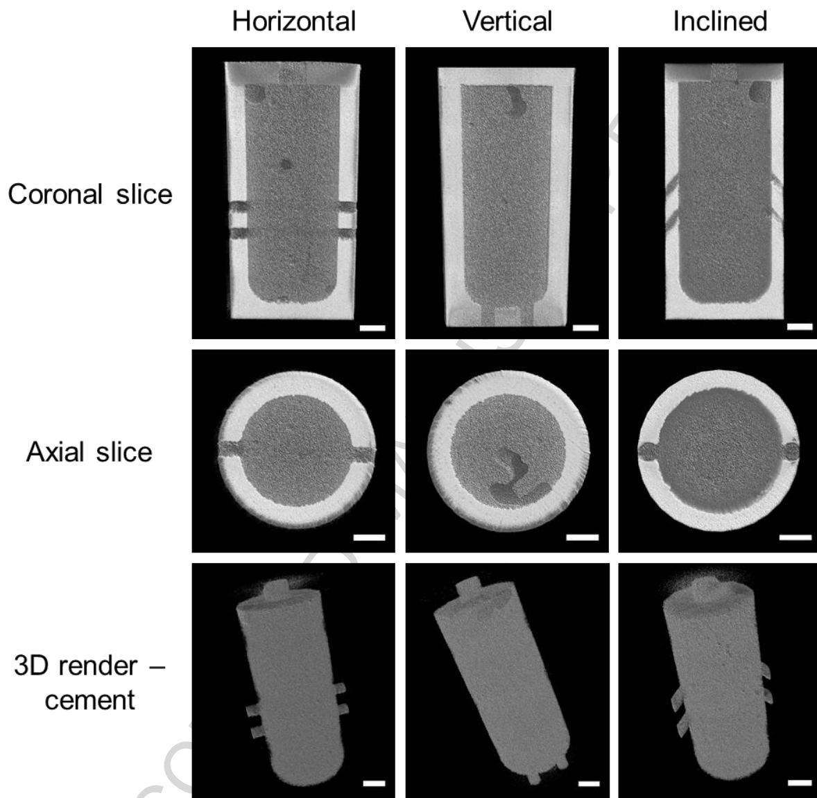
Figure 5: 3D visualisation of gentamicin loaded cement within demonstration implants (scale bars 2 mm)
