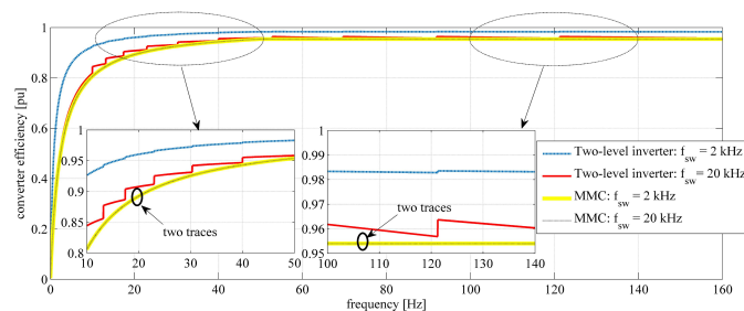
Fig. 6: The efficiency for both topologies versus frequency at full-load current.
