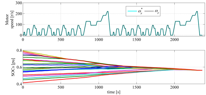
Fig. 12: The motor speed, and SOC of battery cells.
