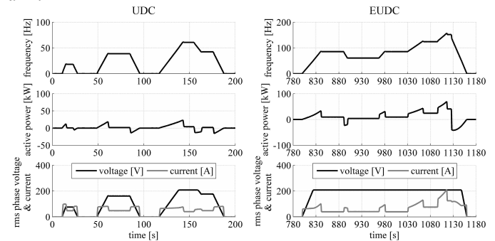
Fig. 9: The motor electric active power, voltage and current.
