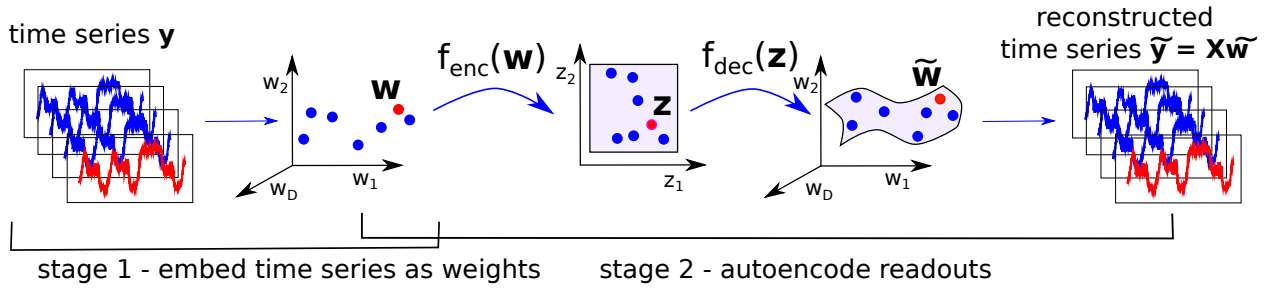
Fig. 1: Sketch of proposed method. In a first stage, time series \mathbf{y} are cast to readout weights \mathbf{w} in the weight space (see Section 3.1). In a second stage, the autoencoder projects readout weights \mathbf{w} onto coordinates \mathbf{z} residing in a two-dimensional space, and reconstructs them again as \tilde{\mathbf{w}} (see Section 3.2). By multiplying with the state space, given by \mathbf{X} , we map the reconstructed readout weights \tilde{\mathbf{w}} to the sequence space where reconstruction error is measured (see Eq. 7).
