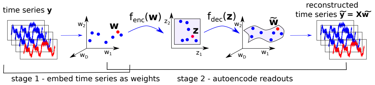
Fig. 1: Sketch of proposed method. In a first stage, time series y are cast to readout weights w in the weight space (see Section 3.1). In a second stage, the autoencoder projects readout weights w onto coordinates z residing in a two-dimensional space, and reconstructs them again as \tilde{w} (see Section 3.2). By multiplying with the state space, given by X , we map the reconstructed readout weights \tilde{w} to the sequence space where reconstruction error is measured (see Eq. 7).
