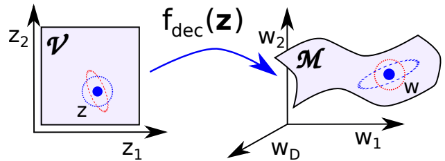
Fig. 3: Stylised sketch: mapping f_{dec}(\mathbf{z}) embeds the visualisation space \mathcal{V} as a manifold \mathcal{M} in the space of readout weights \mathbf{w} . Each point \mathbf{z} addresses a probabilistic ESN with readout weights \mathbf{w} .
