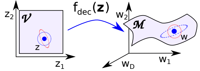
Fig. 3: Stylised sketch: mapping f_{dec}(\mathbf{z}) embeds the visualisation space \mathcal{V} as a manifold \mathcal{M} in the space of readout weights. Each point \mathbf{z} addresses a probabilistic ESN with readout weights \mathbf{w} .
