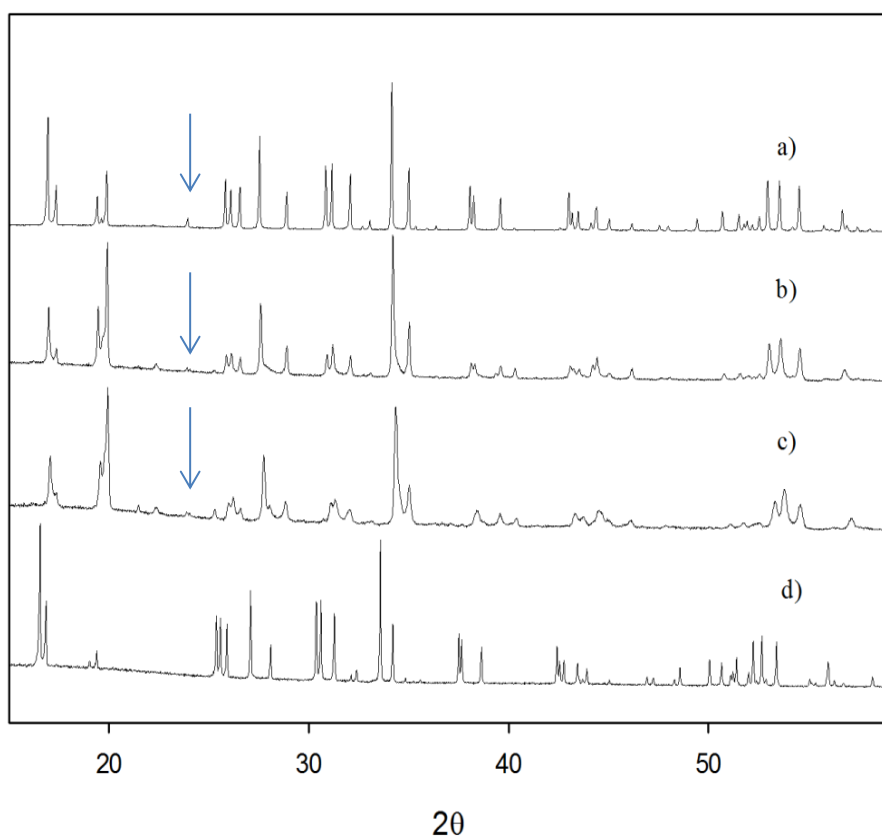
Fig. 1. X-ray diffraction patterns of a) NdSr 2 Ta 2 Li 7 O 12 b) SmSr 2 Ta 2 Li 7 O 12 c) GdSr 2 Ta 2 Li 7 O 12 (arrow indicating impurity Perovskite type phase), and (d) tetragonal La 3 Zr 2 Li 7 O 12 for comparison
