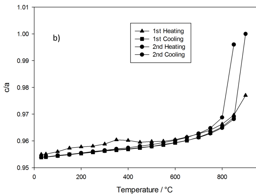
Fig. 4. a) Temperature dependence of the calculated wt%. of cubic phase for \text{PrSr}_2\text{Ta}_2\text{Li}_7\text{O}_{12} b) temperature dependence of tetragonality ( c/a ratio) for the tetragonal \text{PrSr}_2\text{Ta}_2\text{Li}_7\text{O}_{12} phase
