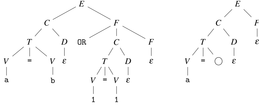
Figure 7: Parse tree for a = b OR 1 = 1 and partial parse tree for a = \bigcirc
