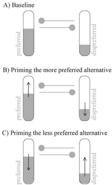
Figure 1. Schematic overview of the mechanisms in the selection stage of the Two-stage Competition model. Sentence production begins with the construction of a message; minimally a thematic structure detailing who does what to whom. Message encoding is followed by a selection stage in which a speaker selects a mapping of the thematic roles to one structural alternative (e.g. actives vs. passives); then follows the planning stage (not shown in the figure) during which production is planned incrementally. While structure choice is determined exclusively during the selection stage, production latency is an additive effect of the time taken in both the selection and planning stages. Between the two structural alternatives there is competition: each node inhibits the other in proportion to its own activation level; the selection time is determined by the amount of time it takes to resolve competition. The selection time thus changes due to priming and the changes differ for preferred and dispreferred structures. Planning time always decreases as a result of priming. Displayed are for the selection stage the (changes in) average activation levels for the preferred (left) and dispreferred (right) structural alternative in three situations. A) The baseline (unprimed) situation. The average base-level activation of each node is positively related to the frequency of occurrence of the corresponding structural alternative. As a consequence of structural priming, the average activation levels of the nodes change; B) Priming the more preferred alternative results in i) an increased difference in activation levels between the nodes, ii) a decreased selection time and iii) a decreased planning time; C) Priming the less preferred alternative results in i) a decreased difference in activation levels between the nodes, ii) an increased selection time and iii) a decreased planning time. The selection time and the planning time contribute to the production latency as additive effects and thus only for preferred structures priming results in speeded response latencies. Note that for actives, which have a highly asymmetrical structure preference relationship with their alternative, priming would not likely affect selection since active are already at a ceiling level.
