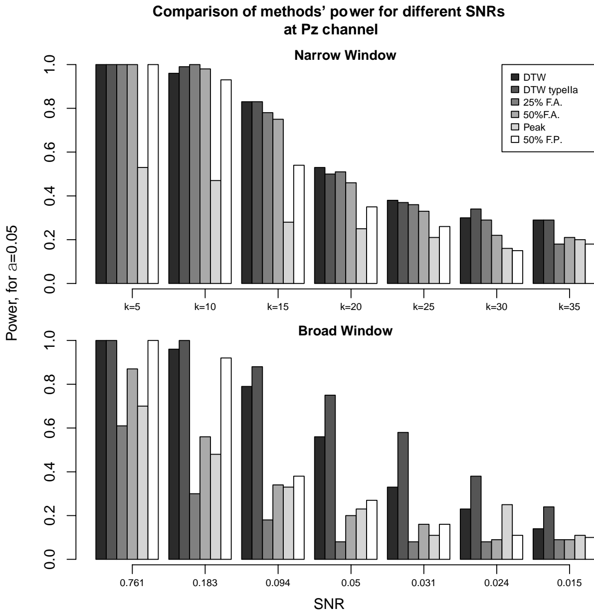
Figure 10: Comparison of the methods' statistical power at channel Pz. For the narrow window, 50% fractional area has the best performance for high SNRs, while DTW and DTW typeIIa have consistently good power. When the broad window is used, 50% fractional area's power significantly reduces, while DTW typeIIa outperforms all methods for all SNRs.
