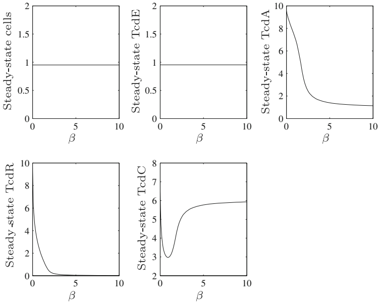
Fig. 4 A steady-state plot of the system in response to changes in \beta ( \epsilon = 0.1 ) if TcdC is produced throughout growth ( F = 1 for all \tau ). We omit extracellular toxin levels from these solutions since they never achieve steady state under our assumptions (as we assume toxins are secreted as long as cells and TcdA are present), but any effect on toxin levels can be inferred from the solution for TcdA (since extracellular toxins are downstream of the rest of the system, this has no consequence on any other variable). Notice that the dip in TcdC levels occurs because TcdC is free (unbound) at low \beta , while for large \beta TcdR is sequestered sufficiently early for TcdC to be produced and remain free in the cell with no additional TcdR to bind. Intermediate values of \beta result in a decrease in TcdC as a result of binding to TcdR. Given that the system is monostable, our simple choice of initial conditions given in Fig. 2 does not affect the steady state of the system
