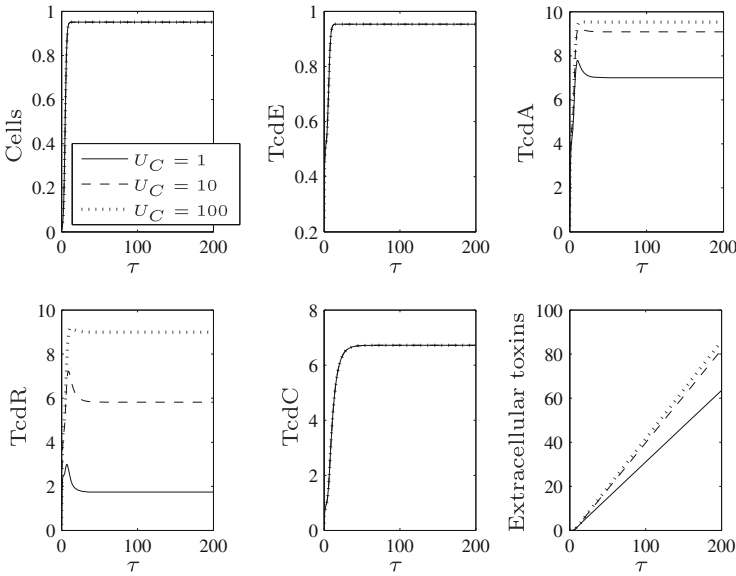
Fig. 6 Time-dependent numerical solution to the full system, assuming TcdC inhibits TcdR on the transcriptional level and is produced throughout growth (Eqs. (10)–(12) and (15)–(17) with \epsilon = 0.1 and F = 1 for all \tau ). The solid line represents full inhibition ( U_C = 1 ), while the dashed ( U_C = O(1/\epsilon) ) and dotted ( U_C = O(1/\epsilon^2) ) lines illustrate an increasing inability for TcdC to bind and block tcdR transcription (i.e. this represents the hypervirulent case). As with the case where TcdC binds TcdR, in this scenario toxin production can be lowered in the long term
