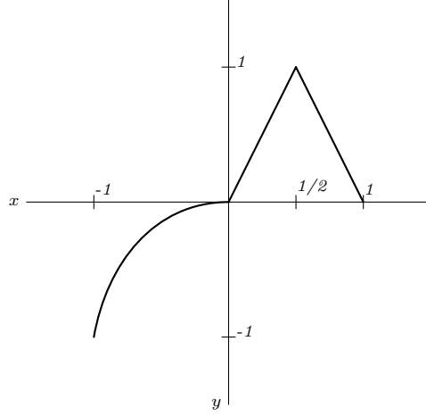
FIGURE 1. The graph of a function f : [-1, 1] \rightarrow [-1, 1] which satisfies ICT(f) = \omega_f but does not exhibit shadowing.
