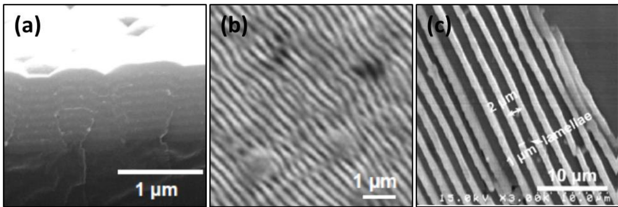
Figure 4. Lithographic replication of butterfly scales. Images of (a) discrete multilayers are formed on the nanopatterned plate by nanocasting lithography. Reproduced with permission. [48] Copyright 2009 Society of Photo Optical Instrumentation Engineers. (b) SEM image of the ripple (nano-groove) pattern made by fs-laser fabrication (after electroforming on Ni plate). Pitch = 300 nm. Reproduced with permission. [49] Copyright 2012 Society of Photo Optical Instrumentation Engineers. (c) Characteristics of butterfly wing: ridge-like structures on replicated scale surface via soft lithography. Reproduced with permission. [35] Copyright 2010 Elsevier B.V.
