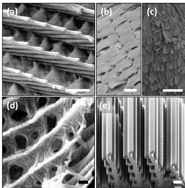
Figure 3. Morpho replication. (a) SEM images of an alumina templated scale, where the replica exhibits fine structures, Scale bar = 1 \mu\text{m} . Reproduced with permission. [25] Copyright 2006, American Chemical Society . (b) SEM image of Morpho rhetenor scales after physical deposition of \text{SiO}_2 , Scale bar = 100 \mu\text{m} . Reproduced with permission. [28] Copyright 2014 Elsevier . (c) SEM image of Morpho menelaus scales after sol-gel deposition of \text{TiO}_2 respectively. Scale bar = 100 \mu\text{m} . Reproduced with permission. [28] Copyright 2014 Elsevier . (d) SEM image of scales exposed to 40 surface sol-gel deposition cycles involving a mixed 2-propanol solution of titanium(IV) isopropoxide and Sn(IV) isopropoxide, Scale bar = 1 \mu\text{m} . Reproduced with permission. [30] Copyright 2008 John Wiley & Sons, Inc. (e) Inclined-view SEM image of Morpho butterfly scale quasi-structure fabricated by FIB-CVD, Scale bar = 1 \mu\text{m} . Reproduced with permission. [12] Copyright 2005 Japan Society of Applied Physics.
