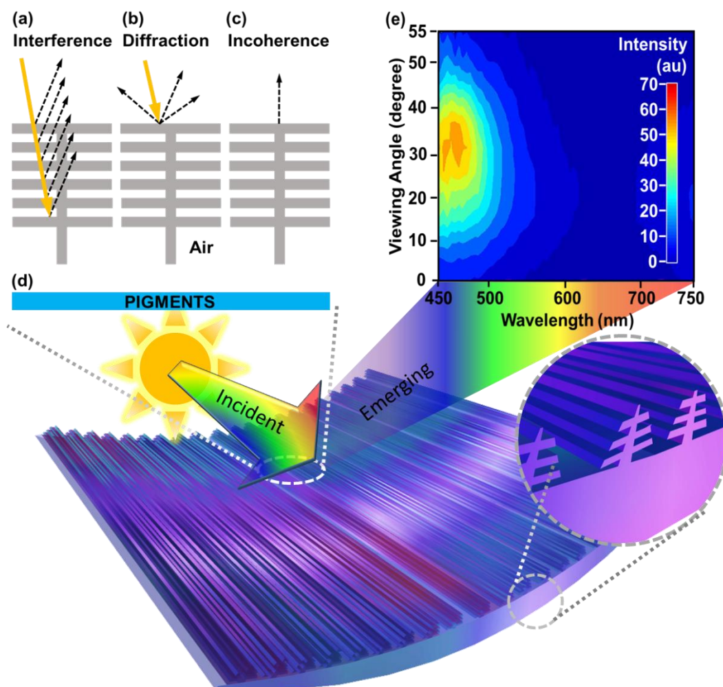
Figure 2. Principles of the blue coloration in the Morpho butterfly. (a) Multilayer interference, (b) Diffraction, and (c) Incoherence (d) Pigment layer (e) Angle-resolved measurements of the back scattered light from Morpho rhetenor . Reproduced with permission. [18] Copyright 2014, Nature Publishing Group.
