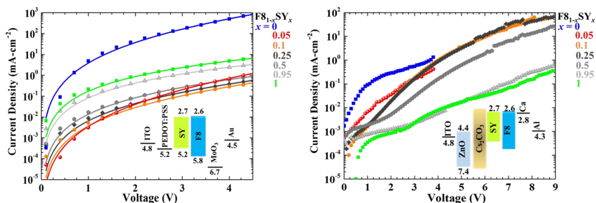
Figure 5. a) J - V curves for F8_{1-x}SY_x based hole only devices with different value of x . The devices are positively biased from the MoO_3 side. The fitting results are shown with solid lines for each curve (see Table 2 ). The current is severely reduced for x = 0.05 and 0.1 indicating hole traps offered by SY molecules. This is because of the large difference present between the HOMOs of F8 and SY. Inset shows the energy band diagram of each layer in the hole only device (Glass/ITO/PEDOT:PSS/ F8_{1-x}SY_x / MoO_3 /Au). The blue dash line in the F8 depicts its \beta -phase LUMO level. b) J - V curves for F8_{1-x}SY_x based electron only devices with increasing SY concentration: The devices are negatively biased from the Ca/Al electrode. There is reduction in electron current for x = 0.05 as compared with pure F8 devices, however at much smaller scale as compared with reduction observed in hole current in hole only devices. Inset shows the energy band diagram of each layer in the electron only device (with schematic Glass/ITO/ZnO/ Cs_2CO_3 / F8_{1-x}SY_x /Ca/Al).
